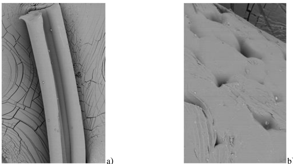
Figure 1. Photos of samples of fibers obtained on installation [8], equipped with reactor with r = 125 mm and 156 dies: a – diameter is 100 \mu\text{m} , magnification is 200 times, b – diameter is 100 \mu\text{m} , magnification is 1000 times, cavities are 1–5 \mu\text{m} .
