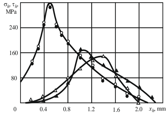
Figure 1. Distribution of contact loads over the flank-land of the cutter in ductile brass (63Cu) machining. \gamma = 0^\circ , \alpha = 18^\circ , \alpha_h = 0^\circ , v = 1.7 m/s, \circ, \bullet – f = 0.06 mm/r; \Delta, \blacktriangle – f = 0.21 mm/r; \circ, \Delta – normal contact load \sigma_h ; \bullet, \blacktriangle – tangential contact load \tau_h . Ordinate – normal \sigma_h [MPa], and tangential \tau_h [MPa] specific contact load over the flank-land; abscissa – distance from the cutting edge on the surface of the flank-land x_h [mm]
