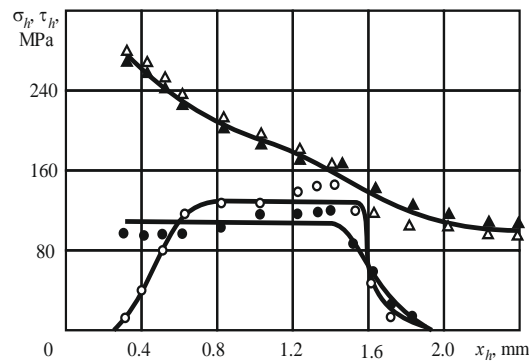
Figure 4. Distribution of contact loads over the flank-land of the cutter in brass machining by the cutter with rounding off cutting edge with radius \rho = 0.3 mm. \gamma = 0^\circ , \alpha = 18^\circ , \alpha_h = 0^\circ , v = 1.7 m/s, \circ , \bullet – ductile brass (63Cu), f = 0.21 mm/r; \Delta , \blacktriangle – brittle brass (57Cu1Al3Mn); f = 0.41 mm/r; \circ , \Delta – normal contact load \sigma_h ; \bullet , \blacktriangle – tangential contact load \tau_h
