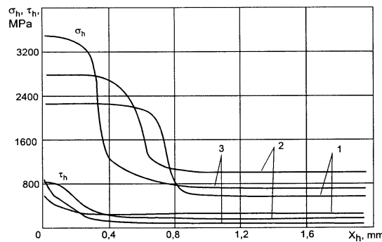
Figure 6. Distribution of normal \sigma_h and tangential \tau_h contact loads over the flank-land of the cutter in titanium alloy cutting without rounding off cutting edge. BT3-1 – BK8, \gamma=0^\circ , \alpha_h=0^\circ , \alpha=10^\circ , v=1 [m/s]: 1 - f=0.11 mm/r; 2 - f=0.21 mm/r; 3 - f=0.41 mm/r. Ordinate – normal \sigma_h [MPa] and tangential \tau_h [MPa] specific contact load on the flank-land; abscissa – distance from the cutting edge on the surface of flank-land x_h [mm].
