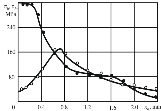
Figure 2. Distribution of contact loads over the flank-land of the cutter in cutting of the ductile brass (63Cu). \gamma = 0^\circ , \alpha = 18^\circ , \alpha_h = 0^\circ , v = 3.6 m/s, f = 0.21 mm/r; \circ – normal contact load \sigma_h ; \bullet – tangential contact load \tau_h . Ordinate – normal \sigma_h [MPa], and tangential \tau_h [MPa] specific contact load over the flank-land; abscissa – distance from the cutting edge on the surface of the flank-land x_h [mm]
