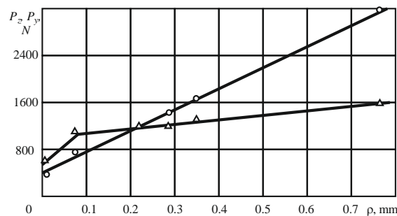
Figure 8. Dependence of cutting force component acting on the rake surface P_{Yr} и P_{Zr} on radius of cutting edge rounding \rho in titanium alloy BT3-1 machining. BT3-1 – BK8, \gamma=0^\circ , \alpha=10^\circ , v=1 m/s, f=0.21 mm/r; \circ - P_{Yr} [N], \Delta - P_{Zr} [N]; machined disk width b=2.3 mm
