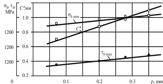
Figure 7. Influence of the cutting edge radius rounding off \rho on the highest contact loads magnitude on the flank-land \sigma_{h \max} , \tau_{h \max} and on the length C' of the horizontal region of the curve \sigma_h in titanium alloy BT3-1 cutting BT3-1 – BK8, \gamma=0^\circ , \alpha=10^\circ , \alpha_h=0^\circ , v=1 m/s, f=0.21 mm/rev; 1 – \rho=0.07 mm; 2 – \rho=0.2 mm; 3 – \rho=0.28 mm; 4 – \rho=0.35 mm; \sigma_h – normal contact load, \tau_h – tangential contact load
