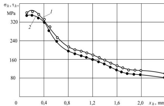
Figure 3. Distribution of normal \sigma_h ( \circ ) and tangential \tau_h ( \bullet ) contact loads over the flank-land of the cutter in cutting of the brittle brass (57Cu1Al3Mn). \gamma = 0^\circ , \alpha = 18^\circ , \alpha_h = 0^\circ , v = 1.7 m/s, f = 0.41 mm/r. Ordinate – normal \sigma_h [MPa], and tangential \tau_h [MPa] specific contact load on the flank-land; abscissa – distance from the cutting edge on the surface of flank-land x_h [mm]
