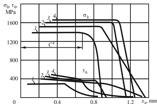
Figure 5. Distribution of contact loads over the flank-land of the cutter in machining of titanium alloy BT3-1 by the cutter with rounding off cutting edge with radius \rho = 0.3 mm. BT3-1 – BK8, \gamma = 0^\circ , \alpha = 10^\circ , \alpha_h = 0^\circ , V = 1 m/s, f = 0.21 mm/r; 1 – \rho = 0.07 mm; 2 – \rho = 0.2 mm; 3 – \rho = 0.28 mm; 4 – \rho = 0.35 mm; \sigma_h – normal contact load on the surface of the flank-land, \tau_h – tangential contact load on the surface of the flank-land
