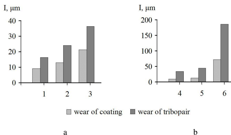
Figure 1. Wear values (I) of tribopairs and coatings under the test load of 25 MPa (a) and 50 MPa (b) and vibratory displacement amplitude: 1 – 30 \mu\text{m} ; 2 – 60 \mu\text{m} ; 3, 4 – 100 \mu\text{m} ; 5 – 150 \mu\text{m} ; 6 – 200 \mu\text{m} .
