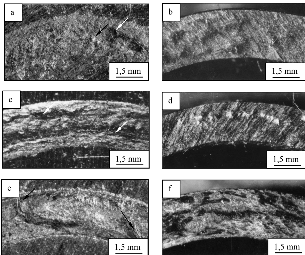
Figure 2. Fragments of coated friction tracks (a, c, e) and counterface (b, d, f). An experiment with amplitude vibratory displacement: a, b – 100 \mu\text{m} ; c, d – 150 \mu\text{m} ; e, f – 200 \mu\text{m} . Arrow marks on the photo show the following: white – cavity; black – adhered wear particles (a) should be abrasive damage (c), burrs (d).
