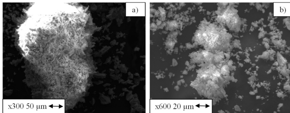
Figure 1. Photographs of the powder mixture ( La_2O_3 + TiO_2 + B ) before mechanical activation at magnification a) of 300 times; b) of 600 times.
