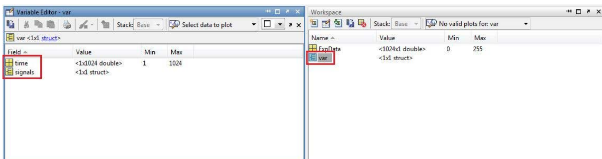
Figure 4. Structure 'var'.
