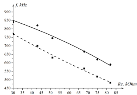
Figure 5. The dependence of the frequency of the output pulses on the value of the resistor in the collector circuit with use of coaxial cable RG64 of various lengths: 5 cm (solid line ●), 10 cm (dashed line ■).
