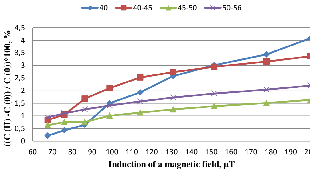
Figure 4. The relative capacity change in the parallel orientations of the external magnetic and measuring electrical fields.
