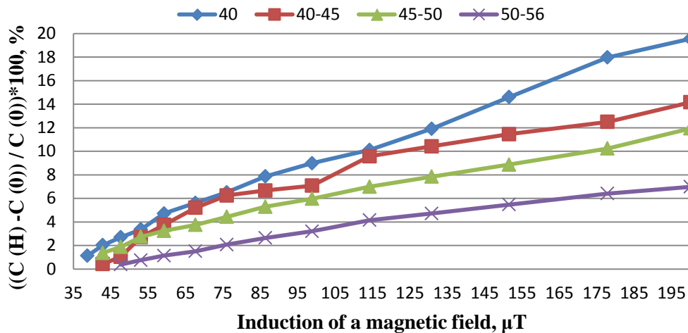
Figure 4. The relative capacity change in the parallel orientations of the external magnetic and measuring electrical fields.
