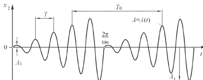
Figure 2. Amplitude modulation with a linear law of the amplitude change: T and T_0 – periods of the carrier and modulating functions, accordingly.
