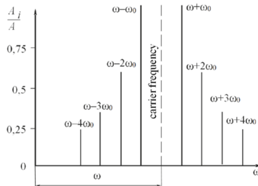
Figure 3. The range of the AM vibrations in the linear modulating function.
