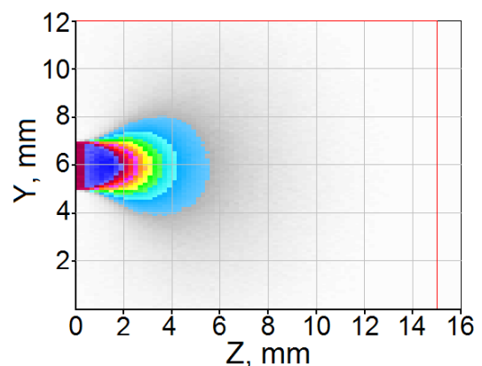
Figure 5. The electron beam distribution in the horizontal plane (the modified ABS-plastic density – 2.5 g/cm 3 ).
