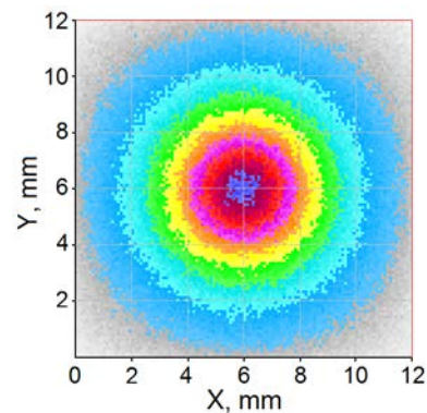
Figure 7. The electron beam shape in the vertical plane at the distance from microtron output window equal to 5 cm (the modified ABS-plastic density – 2.5 \text{ g/cm}^3 ).
