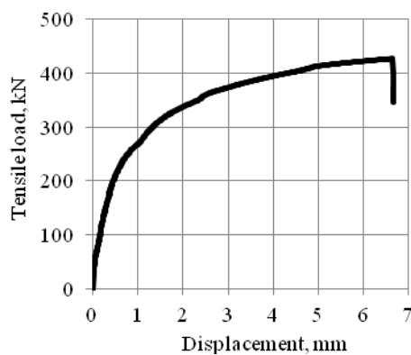
Figure 4. Deformation curve of rebar coupler. Figure 5. Surface deformation of rebar coupler: a – elastic deformation; b – inelastic deformation.
