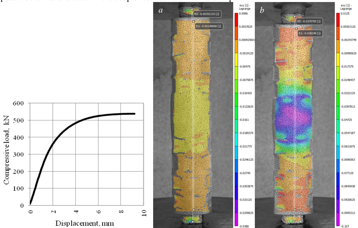
Figure 6. Deformation curve of rebar coupler connection with 20 mm gap.
