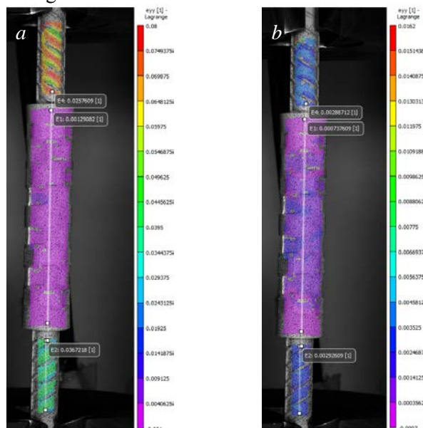
Figure 4. Deformation curve of rebar coupler. Figure 5. Surface deformation of rebar coupler: a – elastic deformation; b – inelastic deformation.
