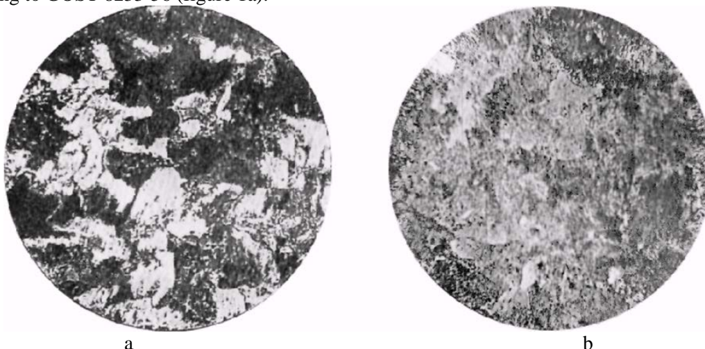
Figure 1. Photo-standards of lamellar pearlite GOST 8233: a – grade 1, b – grade 2.
