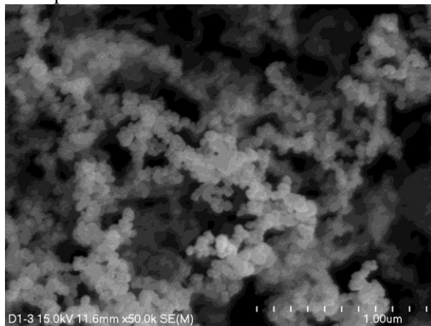
Figure 1C. Complex network of soot particles' aggregates - Sample D1.
