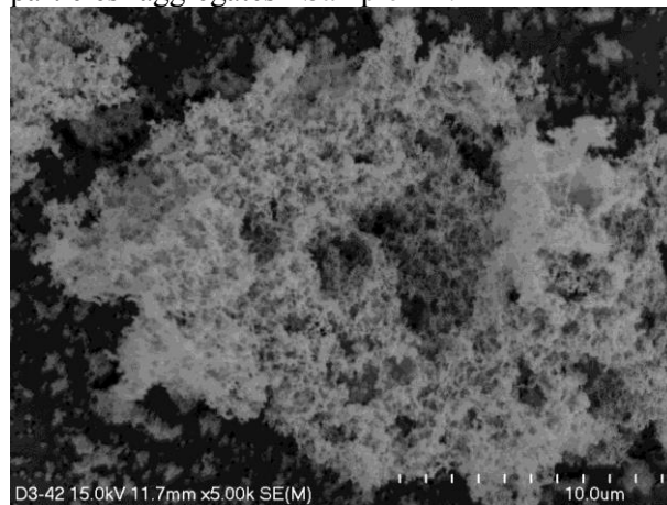
Figure 1F. Isometric aggregate of soot particles - Sample D3.
