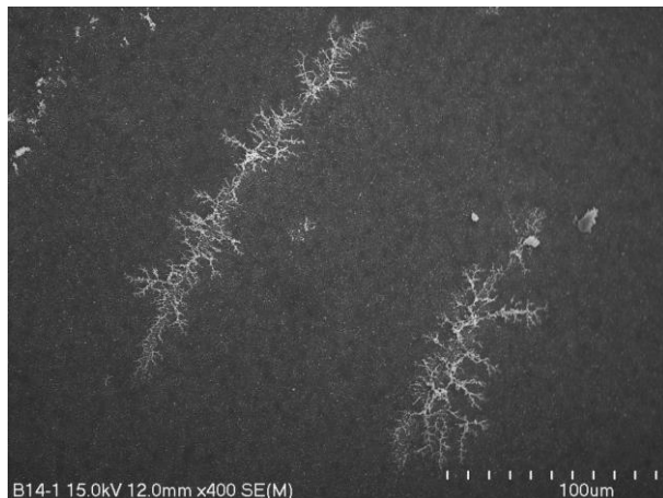
Figure 3C. Chain-like aggregates of soot particles - Sample B14.
