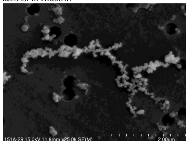
Figure 5D. Chain-like soot particles' aggregate - aerosol in Krakow.
