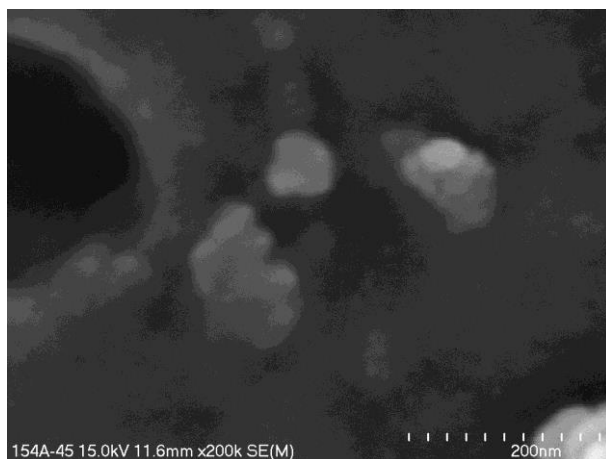
Figure 5A. Single soot particles - aerosol in Krakow.
