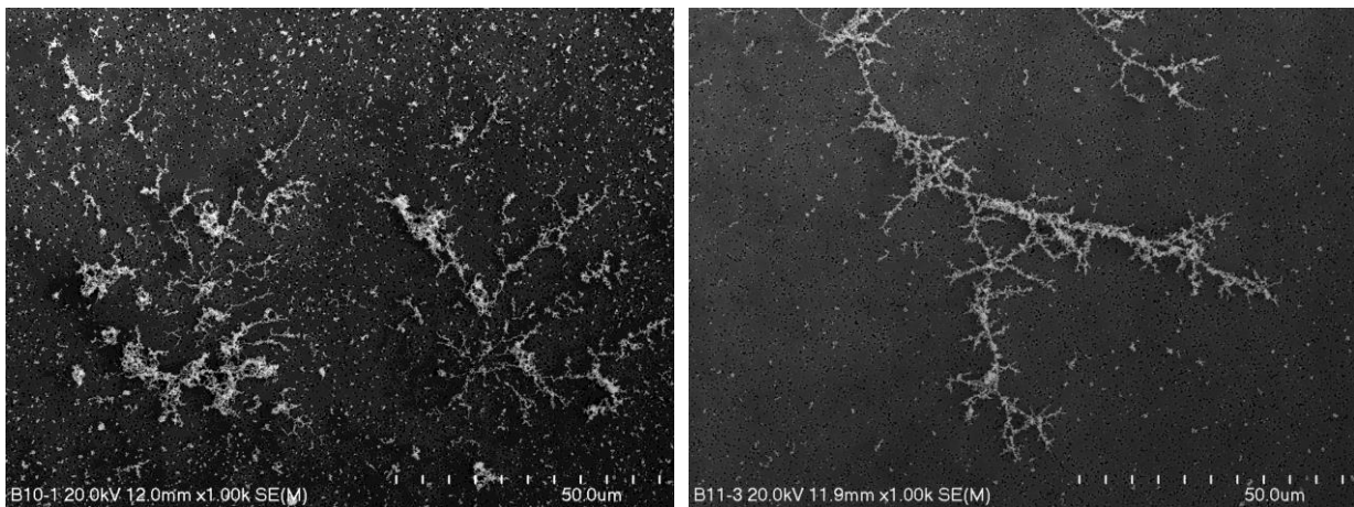
Figure 3A. Single particles and complex aggregates of soot - Sample B10.
