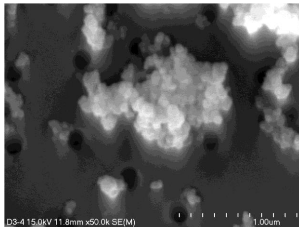
Figure 1B. Soot particles in aggregate - Sample D3.
