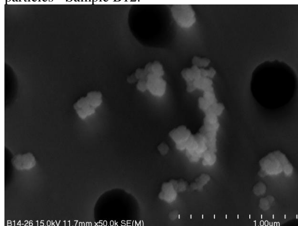
Figure 3F. Single soot particles and small aggregates - Sample B14
