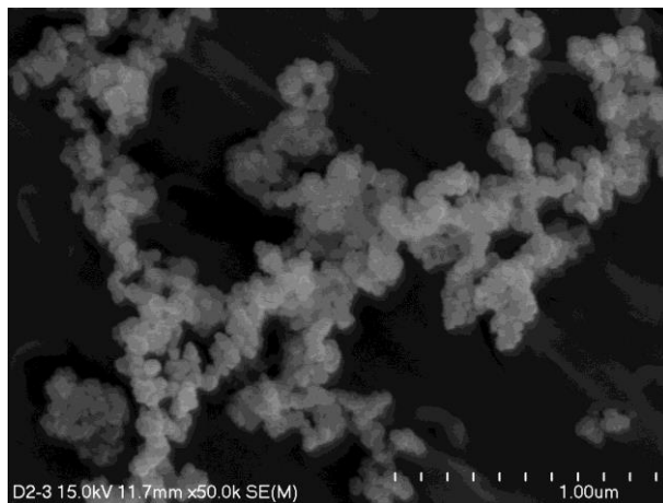
Figure 1A. Soot particles in chain-like aggregate - Sample D2.
