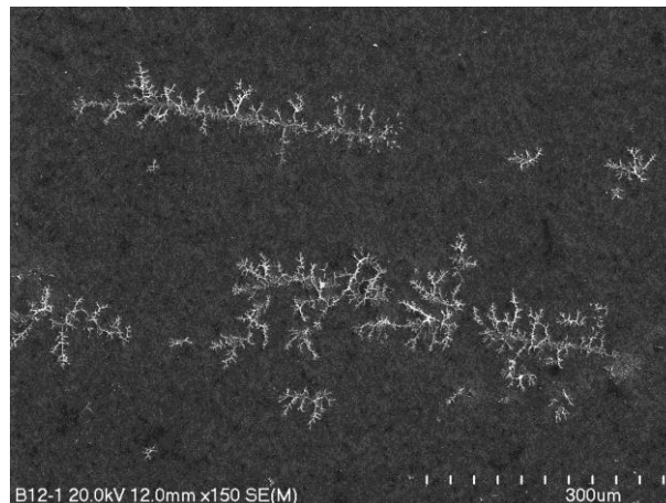
Figure 3D. Chain-like aggregates of soot particles - Sample B12.
