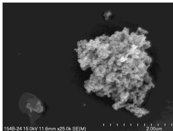
Figure 5F. Densely packed aggregate of soot particles - aerosol in Krakow.
