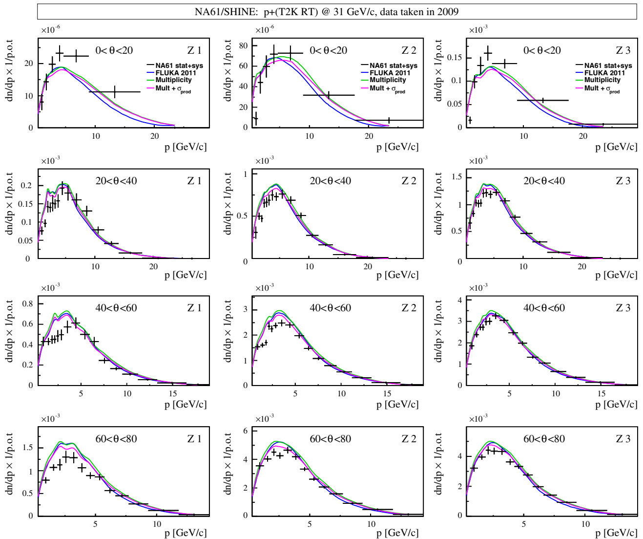
Fig. 22 Spectra of positively charged pions overlaid with nominal FLUKA predictions ( blue ), FLUKA re-weighted for the multiplicities ( green ) and FLUKA re-weighted for multiplicities and production cross
