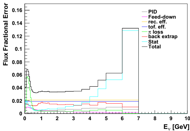
Fig. 29 Propagated statistical and systematic uncertainties for the p+(T2K RT)@31\text{ GeV}/c replica target results for the \nu_\mu flux at SK. The statistical uncertainties are considered as not being correlated between the different NA61/SHINE analysis bins, while for each component of the systematic uncertainties the correlation is considered to be maximal. The different components of the systematic uncertainties are considered as not being correlated between each other
