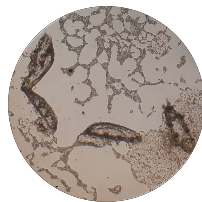
Figure 4: High temp. tardigrades after 1 hour treatment (Dead). 100x
