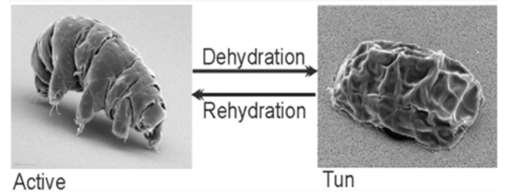
Figure 2: Scanning electron micrograph of active tardigrade versus tun state.
