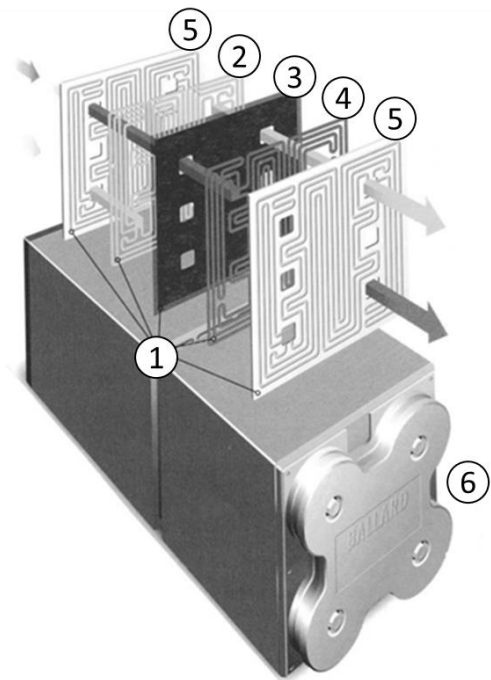
Figure 2. 1: PEFC stack; 2: H 2 flow field; 3: membrane-electrode assembly; 4: air flow field; 5: bipolar plate; 6: endplate [1]
