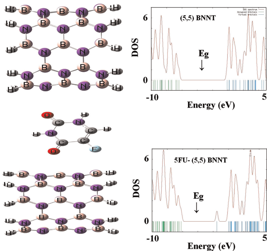
Fig. 2. Optimized structures of (5, 5) BNNT and 5FU/(5, 5) BNNT complex and their density of states.
