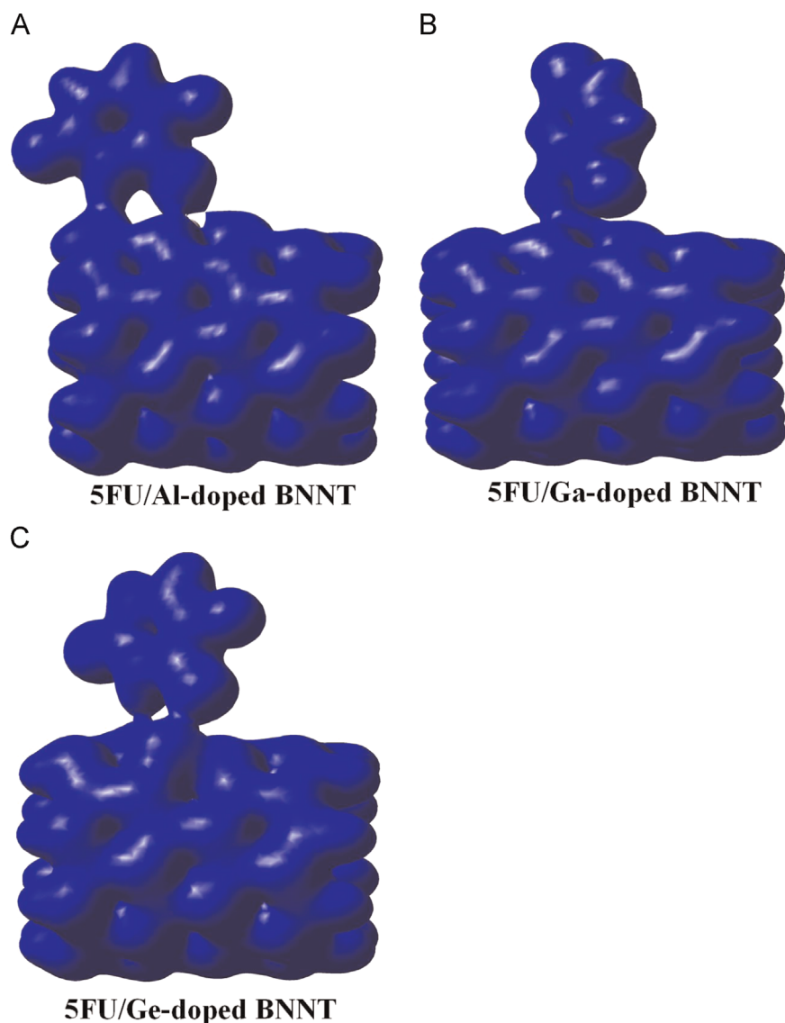
Fig. 6. Iso-surfaces of the total electron density for the 5FU/Al-, Ga-, and Ge-doped BNNTs complexes.
