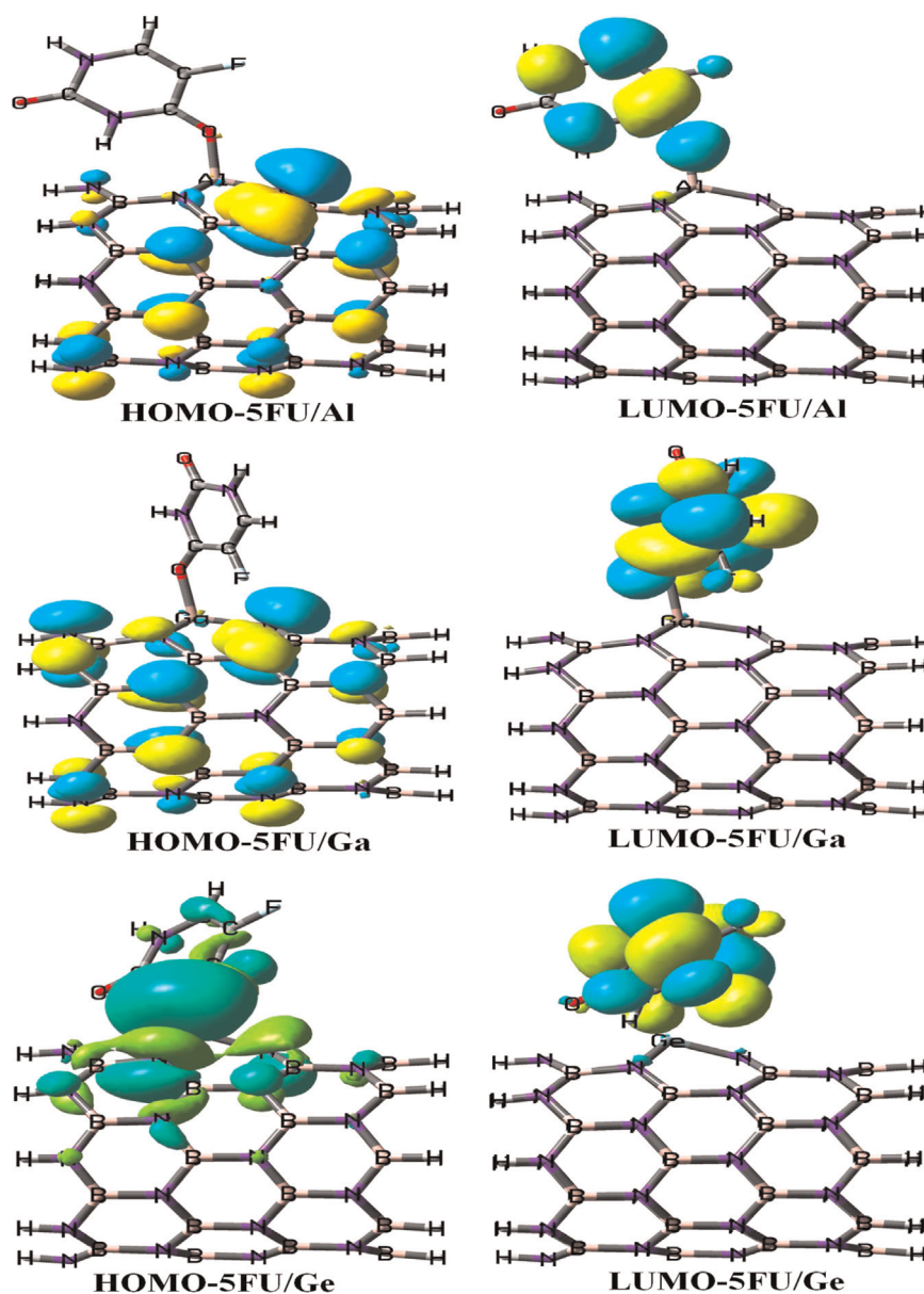
Fig. 4. Charge distributions of HOMO and LUMO orbitals for the 5FU/Al-, Ga-, and Ge-doped BNNTs complexes.
