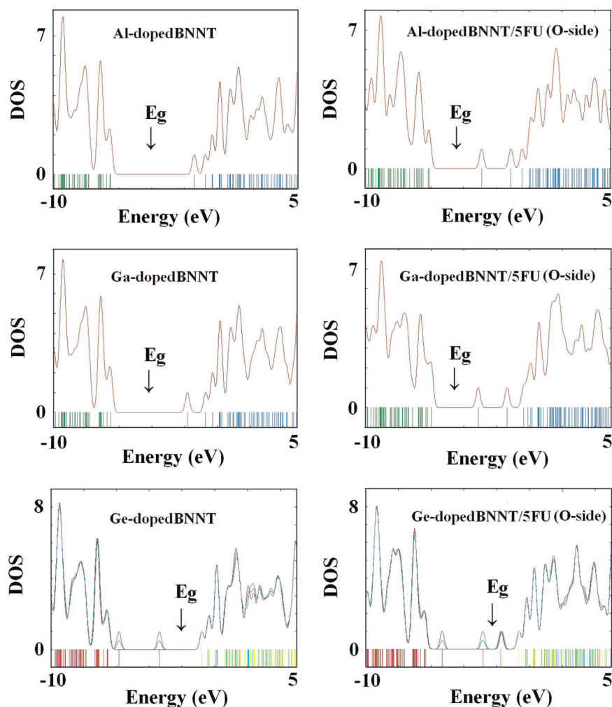
Fig. 5. DOS plots for the applied systems.
