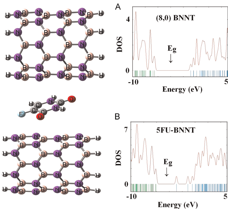
Fig. 1. Optimized structures of (8, 0) BNNT and 5FU/BNNT complex and their density of states.
