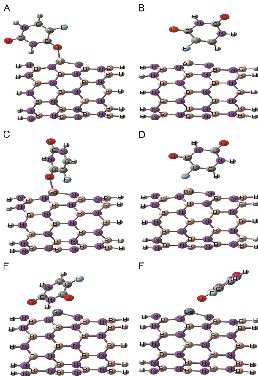
Fig. 3. Optimized configurations for the 5FU molecule upon the Al-, Ga-, and Ge-doped BNNTs.
