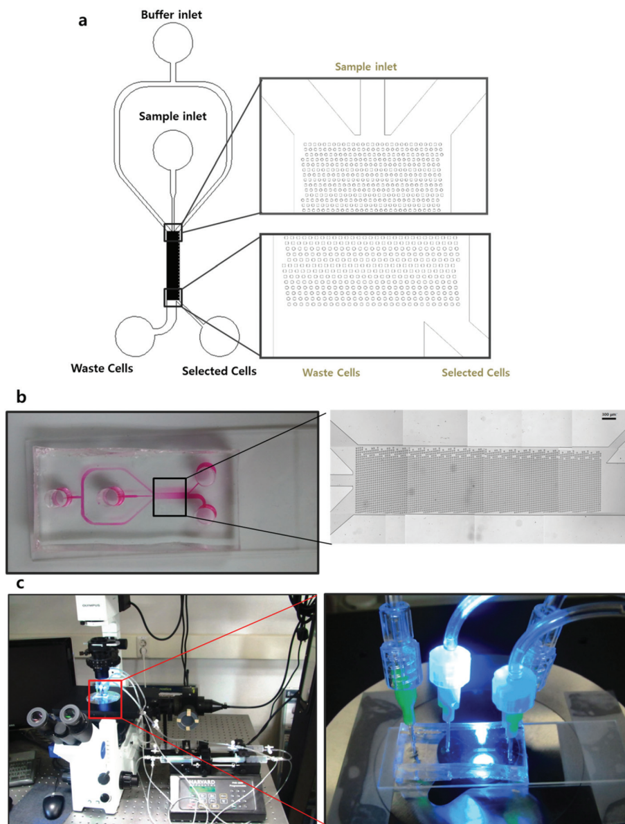
Fig. 2 Microfluidic chip fabrication and experimental setup. (a) CAD drawing of the cell separation system with integrated microposts. (b) Chip fabricated using soft lithography and the overall images of the fabricated microfluidic chip integrated with microposts. (c) Overall experimental setup for cell separation in micropost integrated microchannel and blunt-ended needle connecting the microchip and tube.
