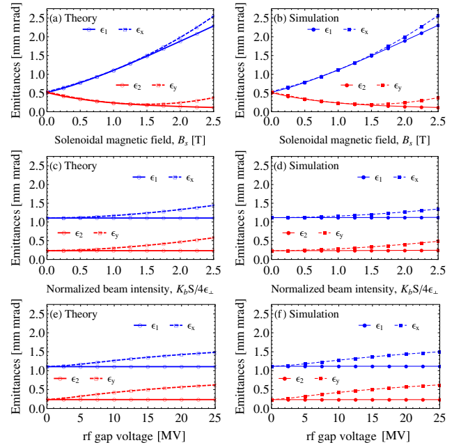
FIG. 1. Plots of the eigenemittances (solid lines with circles) and projected rms emittances (dashed lines with squares) at the exit of the skew-quadrupole triplet. Frames (a), (c), and (e) represent the results of the present KV model analyzed by Mathematica [39], and frames (b), (d), and (f) represent the results of the multiparticle tracking simulations using TRACK code [40]. Frames (a) and (b) correspond to the cases with K_b = 0 and zero acceleration, frames (c) and (d) to the cases with B_s = 1 T and zero acceleration, and frames (e) and (f) to the cases with B_s = 1 T and K_b = 0 , respectively.
