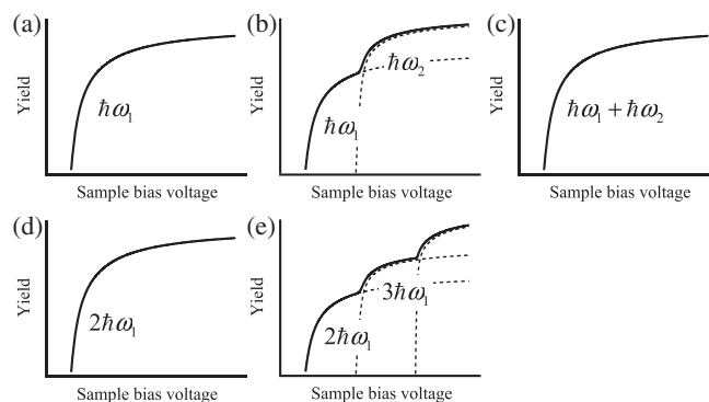
FIG. 1. Schematic illustrations of five types of action spectra: (a) Single-mode excitation; (b) multiple-mode excitation; (c) combination-mode excitation; (d) single-overtone-mode excitation; and (e) multiple-overtone-mode excitation.
