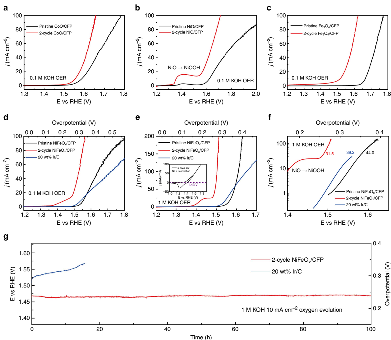
Figure 3 | OER activities and stability of pristine and 2-cycle TMO/CFP catalysts. (a–d) The general efficacy of galvanostatic cycling in improving the OER activities of Co, Ni, Fe and NiFe oxides in 0.1 M KOH. Two-cycle NiFeO x /CFP exhibits better performance than the Ir/C benchmark. (e,f) The OER polarization curves and the corresponding Tafel plots of pristine and 2-cycle NiFeO x /CFP in 1 M KOH. The polarization scanned from positive potential to negative in the inset indicates the onset potential of 2-cycle NiFeO x /CFP at \sim 1.43 V. The Tafel slope of 2-cycle NiFeO x /CFP is 31.5 mV per decade, better than the Ir/C benchmark. (g) Two-cycle NiFeO x /CFP exhibits an excellent OER stability, achieving 10 \text{ mA cm}^{-2} anodic current at only 1.46 V versus RHE for over 100 h without degradation. This is better than the Ir/C benchmark.
