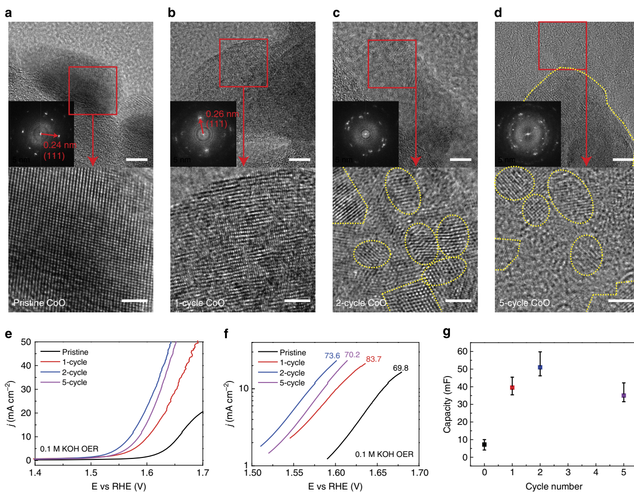
Figure 2 | TEM images and OER activities of battery-cycled CoO/CNF. (a) TEM image of pristine CoO/CNF. The lattice structure and the FFT pattern indicate the single-crystalline nature of the pristine particle. (b) With a blurred lattice orientation still visible, TEM image of 1-cycle CoO/CNF exhibits defects, lattice distortions and expanded (111) spacing. (c) TEM image of 2-cycle CoO/CNF shows the ultra-small, interconnected NPs. The sizes are \sim 2 -5 nm. (d) TEM image of 5-cycle CoO/CNF shows similar domain size to the 2-cycle one. The yellow dash line in the upper image represents the boundary of the whole particle. The zoom-in image indicates the detachment of the ultra-small NPs from the mother particle. Scale bars in a-d , upper, 5 nm; lower, 2 nm. (e) OER catalytic activities of CoO/CNF on CFP in 0.1 M KOH under different galvanostatic cycles. The polarization scan rate is 5 \text{ mVs}^{-1} . Two-cycle CoO/CNF gives the best performance. (f) The Tafel plots of OER polarization curves. (g) Electrochemical double layer capacitance of CoO/CNF under different cycles. The error bars include three identical samples tested for each cycle number.
