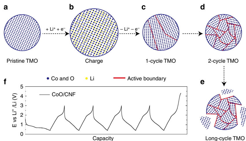
Figure 1 | Schematic of TMO morphology evolution under galvanostatic cycles. (a-e) TMO particles gradually change from single crystalline to ultra-small interconnected crystalline NPs. Long-term battery cycling may result in the break-up of the particle. (f) The galvanostatic cycling profile of CoO/CNF galvanostatic cycling.
