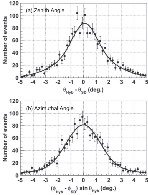
Figure 2. Opening angle distributions of directions measured by hybrid method and SD. Solid curves represent best fits by a double-Gaussian function with the common mean value. (a) Opening angle distributions of zenith angles measured by the hybrid ( \theta_{\text{Hyb}} ) method and the SD ( \theta_{\text{SD}} ). Estimated mean opening angle is m = +0:091 \pm 0:046 . (b) Opening angle of azimuthal angles measured by the hybrid ( \phi_{\text{Hyb}} ) method and the SD ( \phi_{\text{SD}} ). Estimated mean opening angle is m = -0:022 \pm 0:046 . (c) Space angle distribution of direction measured by the hybrid method and the SD. The vertical arrow indicates a space angle containing 68% of the events ( \Delta\alpha = 2:8 \pm 0:1 ).
