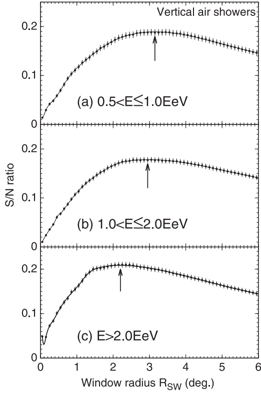
Figure 5. S/N curves for vertical air showers ( \theta < 5^\circ ) as a function of search window size R_{sw} from MC simulation in three energy regions: (a) 0.5 < E(\text{EeV}) \leq 1.0 , (b) 1.0 < E(\text{EeV}) \leq 2.0 , and (c) E(\text{EeV}) > 2.0 . The solid curves are a spline fitting to the MC data as shown by the points. Noise ( =\sqrt{B} , square root of number of background events) is proportional to the area of the search window \pi R_{sw}^2 . Peak (solid arrow) indicates optimal search window radius to maximize S/N.
