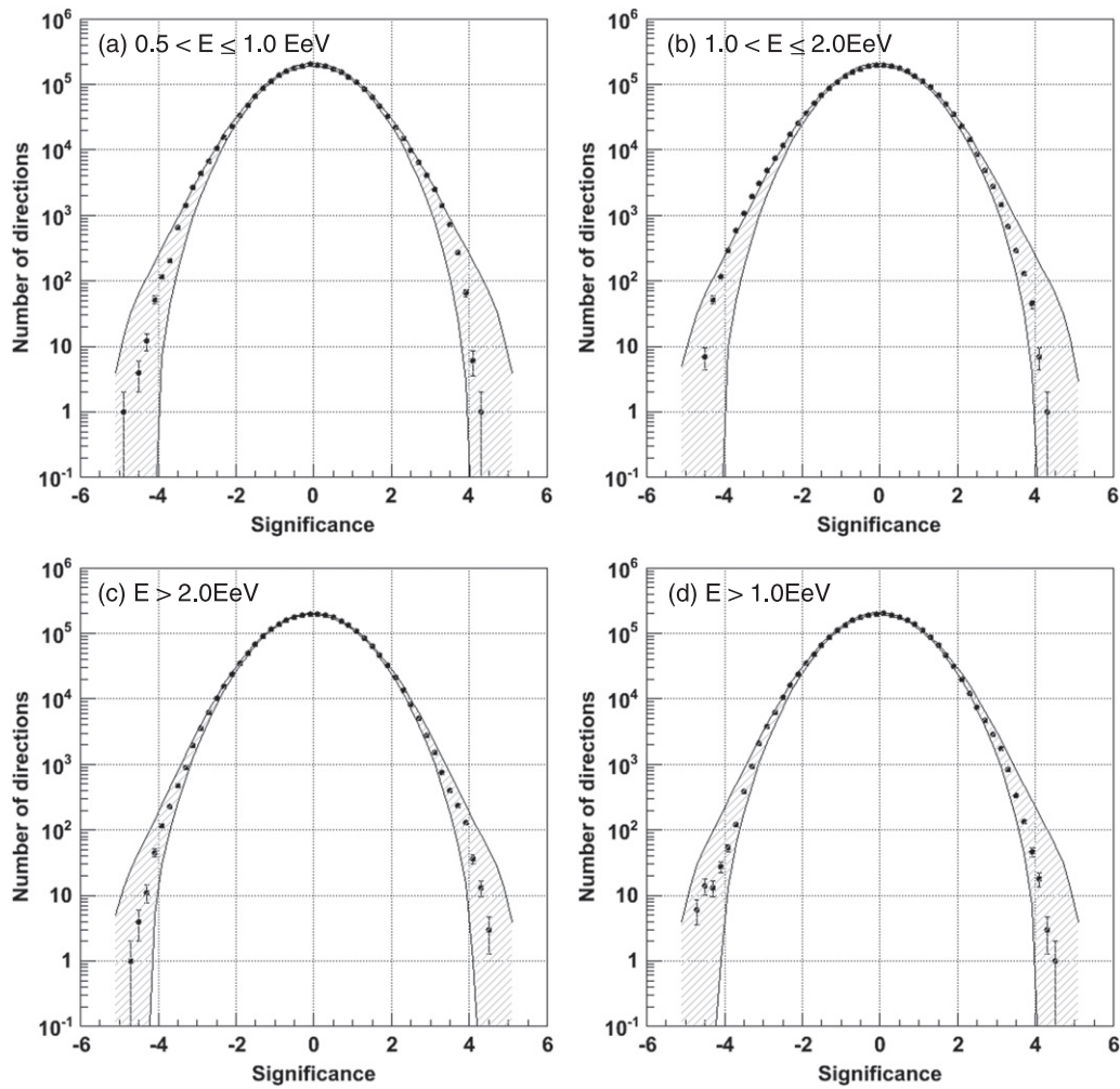
Figure 8. Histograms showing significance distributions in all directions within the FOV of TA SD in four energy regions: (a) 0.5 < E(\text{EeV}) \leq 1.0 , (b) 1.0 < E(\text{EeV}) \leq 2.0 , (c) E(\text{EeV}) > 2.0 , (d) E(\text{EeV}) > 1.0 . The shaded area indicates a 95% containment region of 10^5 MC samples of isotropic sky.
