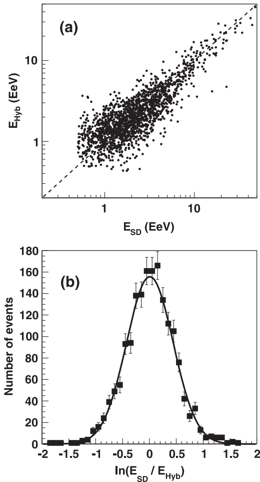
Figure 4. Comparison of reconstructed energies from the SD and hybrid method. (a) Scatter plot of reconstructed energy from the SD and hybrid methods. (b) Natural logarithm of ratio of reconstructed energy from the SD and hybrid methods. Energy resolution with loose-cut data is estimated to be \pm_{-35}^{+50}\% .
