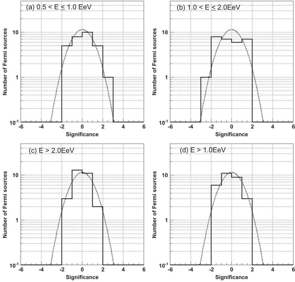
Figure 9. Histograms showing significance distributions of 29 Fermi bright Galactic sources within the FOV of TA SD in four energy regions: (a) 0.5 < E (\text{EeV}) \leq 1.0 , (b) 1.0 < E (\text{EeV}) \leq 2.0 , (c) E (\text{EeV}) > 2.0 , and (d) E (\text{EeV}) > 1.0 . Dotted curves are the expected normal Gaussian distributions.
