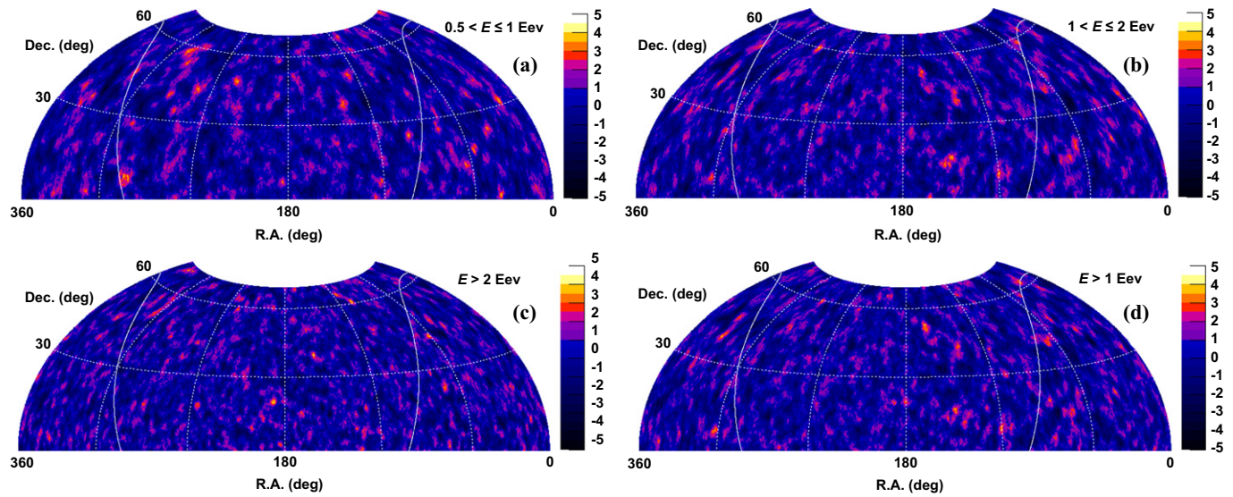
Figure 7. Significance maps of the northern sky between decl. = 0^\circ and decl. = 70^\circ surveyed by TA SD in four energy regions: (a) 0.5 < E(\text{EeV}) \leq 1.0 , (b) 1.0 < E(\text{EeV}) \leq 2.0 , (c) E(\text{EeV}) > 2.0 , and (d) E(\text{EeV}) > 1.0 . Color contours show significance levels. Solid curves indicate the Galactic plane.
