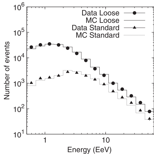
Figure 1. Reconstructed energy distributions. Closed circles and triangles show energy distributions of experimental data after loose and standard cuts, respectively. Solid and dashed histograms show energy distributions in MC simulation after loose and standard cuts, respectively. The areas of MC simulation are normalized to those of the data.
