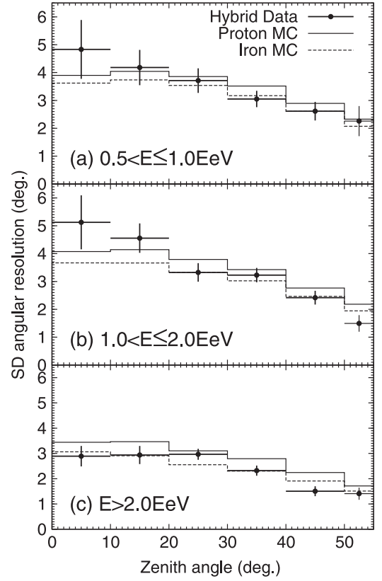
Figure 3. Angular resolutions of TA SD as a function of zenith angle. Solid histograms show results of the MC simulation assuming pure protons. Dashed histograms show results of the MC simulation assuming pure iron. Closed circles indicate the estimated angular resolution from opening angles of reconstructed directions between the SD and hybrid data. Zenith angle of the hybrid data is limited to 55^\circ . The MC simulation and hybrid data are divided into three energy regions: (a) 0.5 < E(\text{EeV}) \leq 1.0 (upper panel), (b) 1.0 < E(\text{EeV}) \leq 2.0 (middle panel), and (c) E(\text{EeV}) > 2.0 (lower panel).
