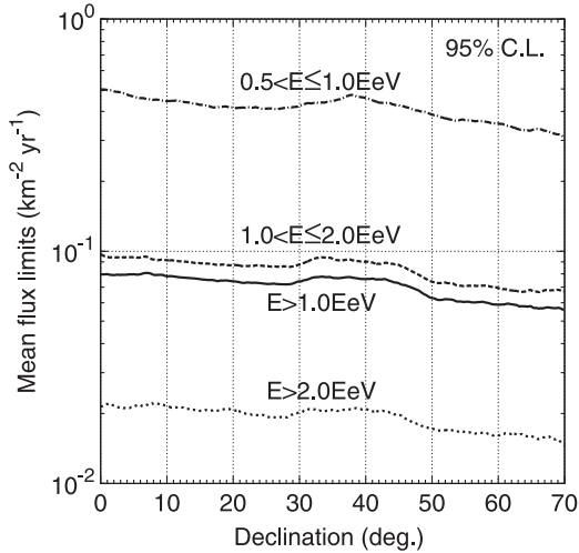
Figure 10. Mean flux upper limits ( \text{km}^{-2} \text{yr}^{-1} ) at 95% confidence level according to the declination of the target sources observed by TA SD at each energy. Dotted-dashed curve: 0.5 < E (\text{EeV}) \leq 1.0 ; dashed curve: 1.0 < E (\text{EeV}) \leq 2.0 ; dotted curve: E (\text{EeV}) > 2.0 ; solid curve: E (\text{EeV}) > 1.0 .
