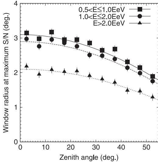
Figure 6. Optimal search window radius as a function of zenith angle \theta from the MC simulation. The curves show the best fit by the empirical formula R_{sw} = R_0 \cos \theta . Symbols and line types represent three different energy regions: squares with solid curve, 0.5 < E(\text{EeV}) \leq 1.0 ; circles with dotted curve, 1.0 < E(\text{EeV}) \leq 2.0 ; and triangles with dashed curve, E(\text{EeV}) > 2.0 .
