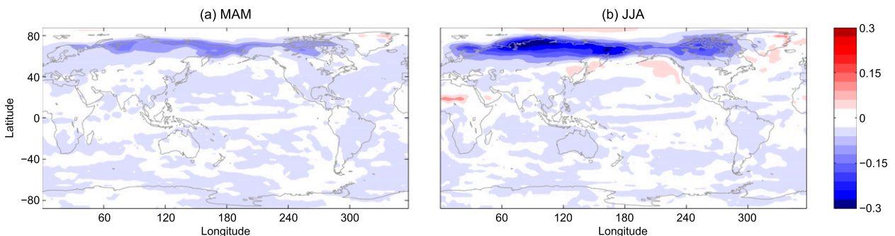
FIG. 8. The response of low cloud amount in (a) MAM and (b) JJA.
