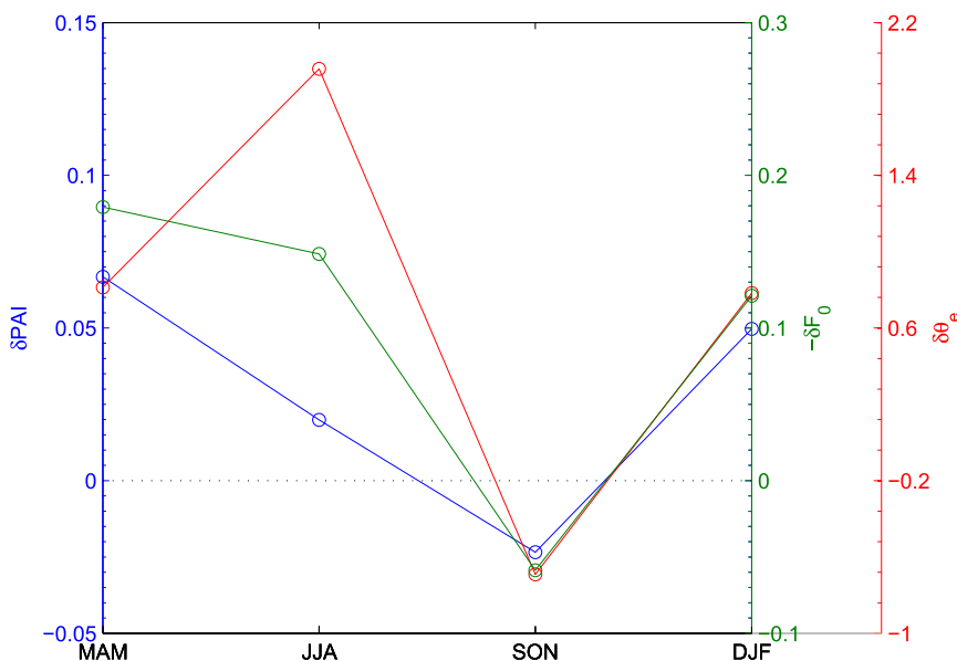
FIG. 3. The difference between VEG and CNT in precipitation asymmetry index \delta\text{PAI} (blue), negative of atmospheric energy transport between 15^\circ\text{S} and 15^\circ\text{N} ( -\delta F_0 ) in PW (green), and energy flux equator \delta\theta_e in degrees (red).
