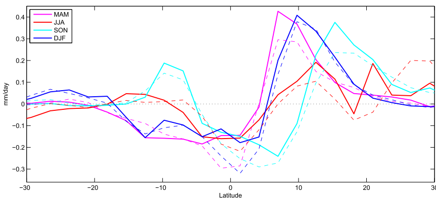
FIG. 4. The zonal-mean response of precipitation (solid) and -\overline{[q_{\text{CNT}} \nabla \cdot \delta \mathbf{v}]} (dashed) between 30^\circ\text{S} and 30^\circ\text{N} in MAM, JJA, SON, and DJF in magenta, red, cyan, and blue, respectively.
