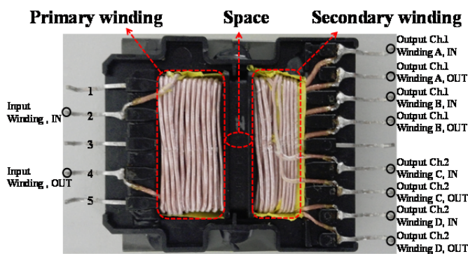
Fig. 2. A transformer for a dual-output half-bridge inductor-inductor-capacitor (LLC) resonant converter.
