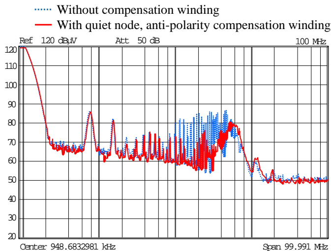
Fig. 12. Measurement results of common mode (CM) noise voltage spectrums.
