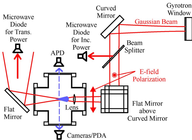
FIG. 1. (Color online) Schematic of breakdown experiment.
