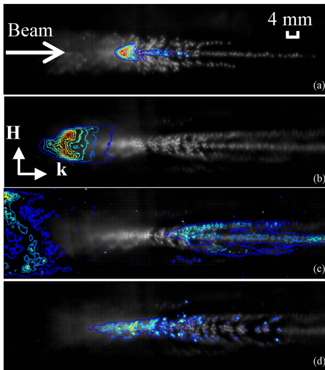
FIG. 10. (Color online) Helium at 730 Torr with 6 ns optical gate pulse starting at (a) t=40 ns, (b) 130 ns, (c) 650 ns, and (d) 2.48 \mu\text{s} .
