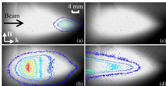
FIG. 11. (Color online) Helium at 1.2 Torr with 6 ns optical gate pulse starting at (a) t=40 ns, (b) 160 ns, (c) 1.14 \mu\text{s} , and (d) 1.92 \mu\text{s} .
