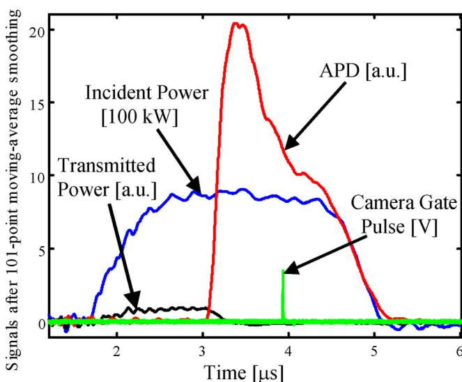
FIG. 2. (Color online) Sample traces of APD, fast camera gate pulse, microwave diode signals for incident and transmitted power, for a pulse with a gas breakdown event. Note that the units differ for each trace.
