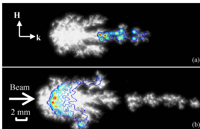
FIG. 8. (Color online) SF 6 at 195 Torr with 6 ns optical gate pulse starting at (a) t=110 ns and (b) 1.34 \mu\text{s} .
