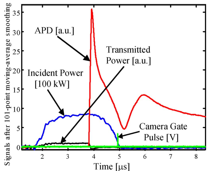
FIG. 12. (Color online) Oscilloscope traces of APD, camera gate pulse, microwave diodes for incident, and transmitted power for the shot shown in Fig. 10(c).
