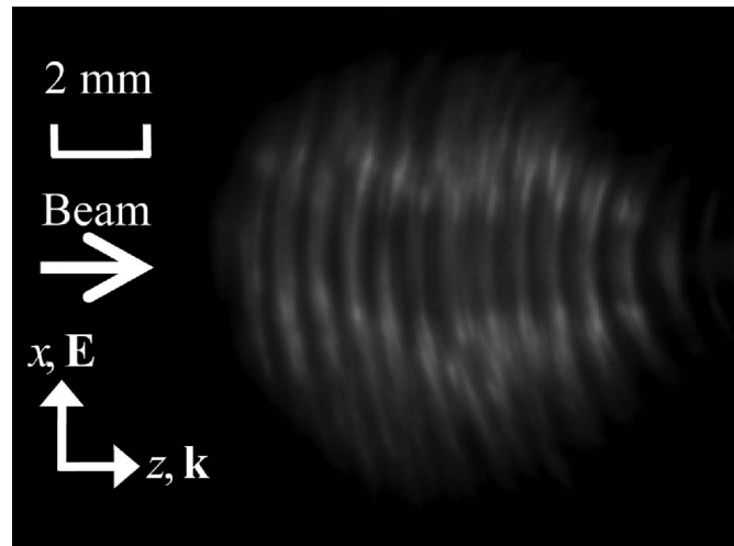
FIG. 3. Typical image captured by the slow camera in ambient air breakdown, viewing in the plane containing E and k (the E -plane). Note the development of the filaments along the direction of the E field.
