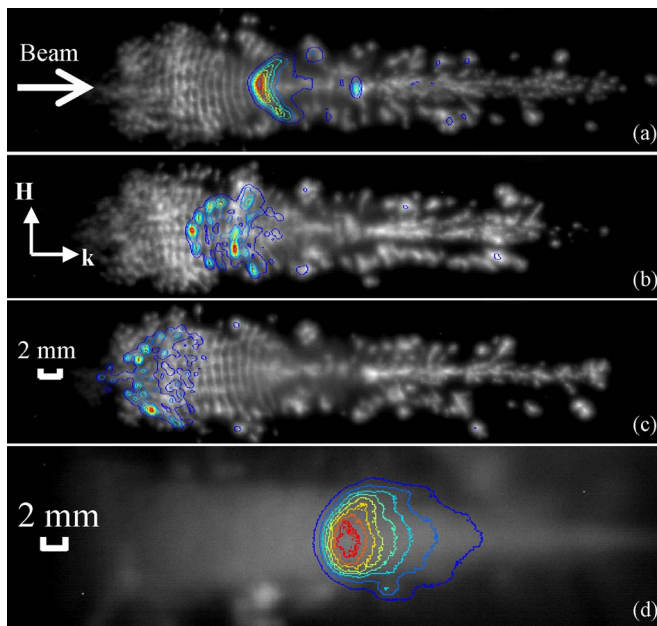
FIG. 7. (Color online) Nitrogen at 360 Torr with 6 ns optical gate pulse starting at (a) t=170 ns, (b) 620 ns, and (c) 1.41 \mu\text{s} , and at 2 Torr with 6 ns long optical gate pulse starting at (d) 100 ns. The scale shown in (c) applies to (a)–(c).
