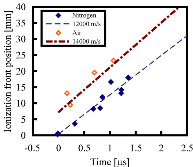
FIG. 13. (Color online) Ionization front position vs gate pulse delay in air and nitrogen at atmospheric pressure for incident power intensity of \sim 3 MW/cm 2 . The dotted lines show the fit for the propagation speed of the ionization front.
