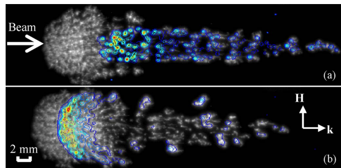
FIG. 9. (Color online) SF 6 at 115 Torr with 6 ns optical gate pulse starting at (a) t=220 ns and (b) 1.45 \mu\text{s} .
