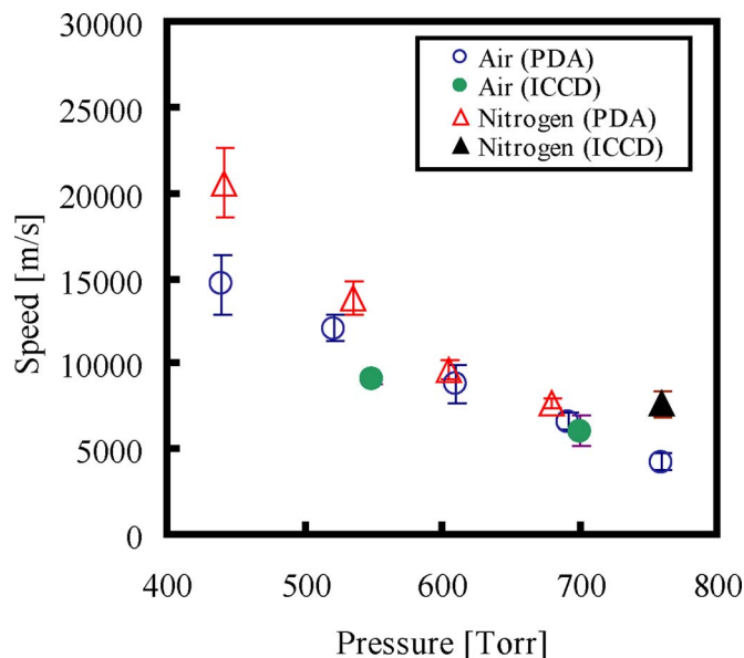
FIG. 14. (Color online) Ionization front propagation speed vs pressure for a microwave beam intensity of 1.5–2 MW/cm 2 . PDA and ICCD values are estimated from the PDA signals and from the fast camera images, respectively.
