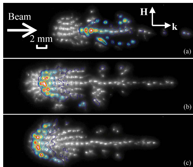
FIG. 4. (Color online) Images of breakdown in ambient air at 710 Torr with 49 ns optical gate pulse starting at (a) t=400 ns, (b) 1.28 \mu\text{s} , and (c) 1.52 \mu\text{s} . The image is taken in the plane containing H and k , the H -plane.
