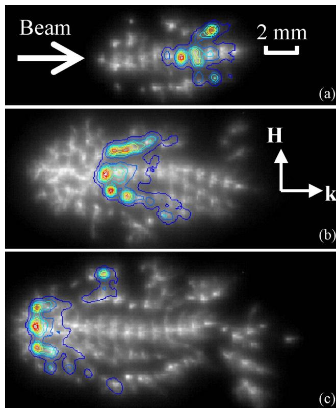
FIG. 6. (Color online) Nitrogen at 780 Torr with 6 ns optical gate pulse starting at (a) t = 360 ns, (b) 710 ns, and (c) 1.25 \mu s.
