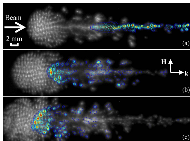
FIG. 5. (Color online) Ambient air at 440 Torr with 49 ns optical gate starting at (a) t = -40 ns, (b) 480 ns, and (c) 720 ns.
