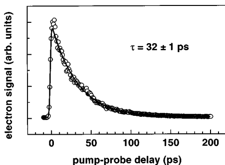
FIG. 12. The decay trace for the S_1 6a_0^2 state, obtained from the spectrum in Fig. 11, with a lifetime of 32 ps. It is known that the S_1 state of pyridin decays by internal conversion to the ground state.
