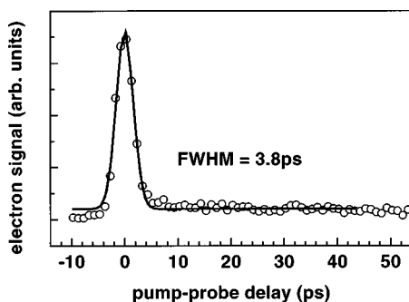
FIG. 13. In the photoelectron spectrum of pyridin a peak at 550 ns due to fast electrons originating from a [3'+1] process can be identified. Analyzing that peak as a function of the pump-probe delay yields the zero in time as well as the instrument response function.
