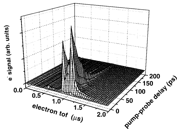
FIG. 11. Time-resolved photoelectron spectrum of the S_1 6a_0^2 state of pyridine, recorded for calibration of our setup. Note the presence of a small peak around t=0 , at an electron time-of-flight of 550 ns.
