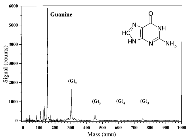
FIG. 5. Typical mass spectrum of kHz rate laser ablated guanine monomer and molecular clusters, resonantly ionized at 277 nm using 150 fs laser pulses. The count rate was 0.3 counts per laser shot (i.e., 300 counts per second), a respectable signal for many purposes. Peaks marked by an asterisk correspond to loss of the \text{NH}_2 group ( m=135 amu) and loss of \text{N}_2\text{CH}_2 ( m=109 amu) from the guanine monomer. For details, see the text.
