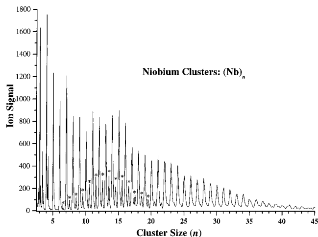
FIG. 4. Typical mass spectrum, recorded in 5 min, of kHz rate laser ablated niobium clusters, nonresonantly ionized at a laser intensity of 1 \times 10^{13} \text{ W/cm}^2 ( \lambda = 0.8 \mu\text{m} ). With this particular growth channel, a broad cluster distribution is obtained with this method. The mass peaks marked by an asterisk are the doubly charged cluster species. This kHz source is stable for over 12 continuous hours of operation. For details, see the text.
