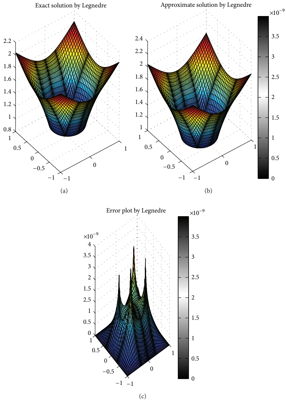
FIGURE 4: Exact solution, approximation solution, and its error for N = 18 .
