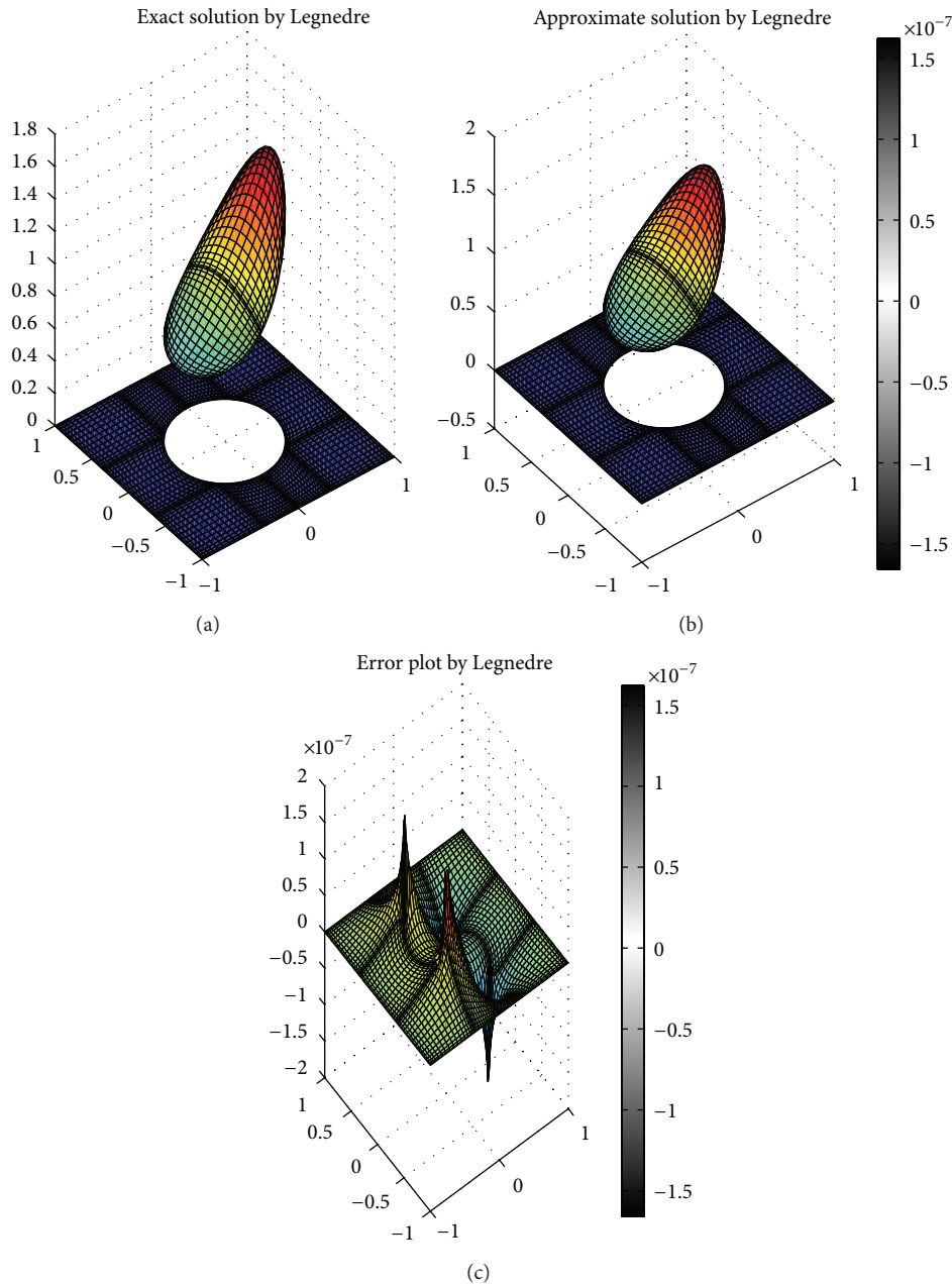
FIGURE 7: Exact solution, approximation solution, and its error for N = 18 .
