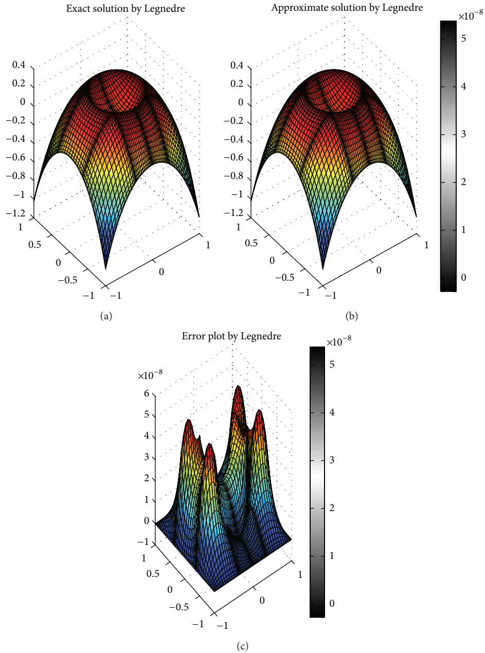
FIGURE 5: Exact solution, approximation solution, and its error for C = 0.1 and b = -3 .
