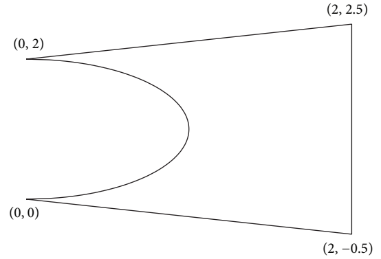
FIGURE 2: A curved domain.
