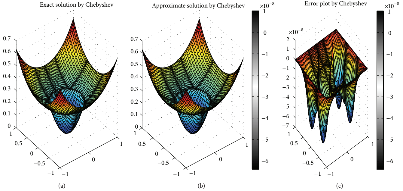
FIGURE 6: Exact solution, approximation solution, and its error for C = 0.1 and b = 10 .
