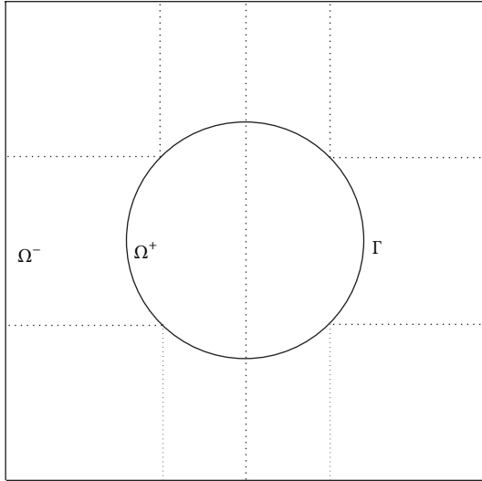
FIGURE 3: Domain decomposition for the interface examples.
