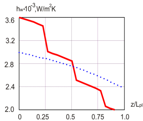
Figure 6: Distribution of local film transfer coefficients at water side along the channel length z .
