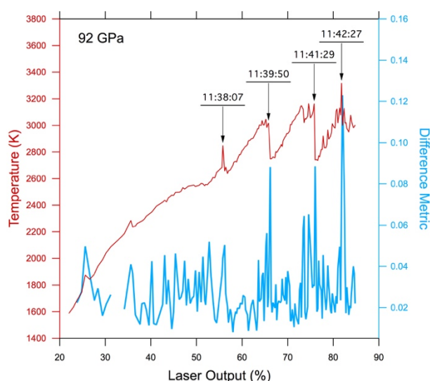
Fig. S1: Power versus temperature data and difference metric measured using 4-colour imaging radiometry at 92 GPa. The timestamps relate to video VS1.
