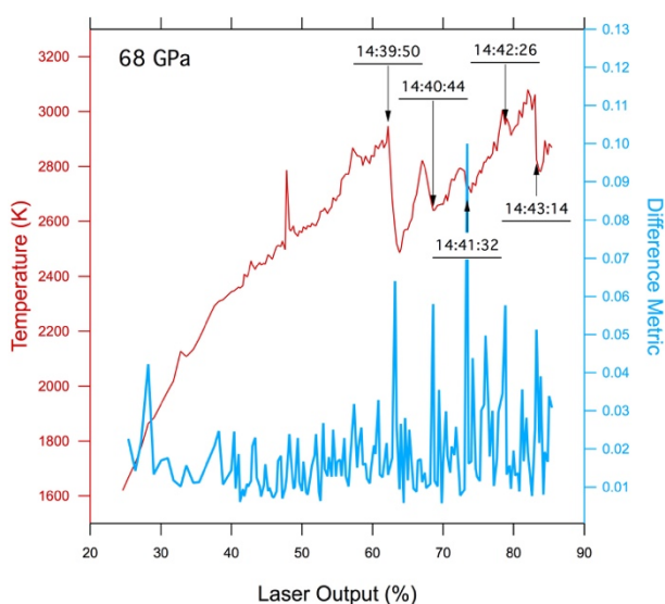
Fig. S2: Power versus temperature data and difference metric measured using 4-colour imaging radiometry at 68 GPa. The time stamps relate to video VS2.
