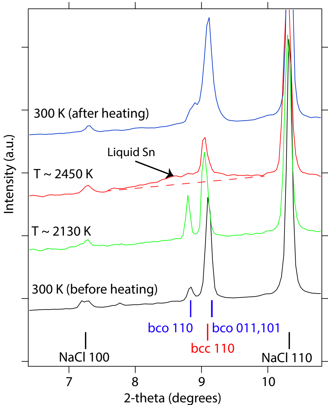
FIG. 5: X-ray diffraction data for \gamma -Sn in the region of the bco 011, 101 and 110 reflections and the bcc 110 reflection. Diffraction data shown were obtained at an initial pressure of 46 GPa during laser heating experiments showing the persistence of the coexisting bco and bcc reflections up to at least 2130 K, just below the melting temperature. The small shift of the peaks to larger d spacing with increasing temperature occurs due to thermal expansion. After quenching from the liquid to room temperature, the bco and bcc reflections both remain present. There is a small broadening of the peaks (increase of \sim 0.03 degrees in peak width of bcc 110 & bco 011, 101 peaks) in the quenched diffraction profile. The quenched sample is at slightly higher pressure and as a consequence the bco peaks are closer together and the bcc peak is more pronounced at the expense of the bco 011, 101 peak intensities. These results are in accordance with the results presented in the room temperature compression study of Salamat et al. [5] The weak peaks near 7.7 degrees
