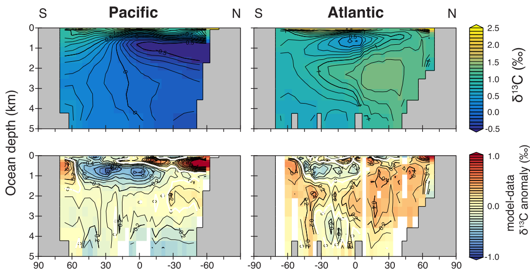
Fig. 1. Evaluation of the global \delta^{13}\text{C} cycle in cGENIE. Shown in the top two panels for present-day Atlantic (right) and Pacific (left) basins, is the zonally-averaged \delta^{13}\text{C} profile of DIC corresponding to year 1998. In the lower two panels are the corresponding zonal anomalies of model year 1998 minus observed \delta^{13}\text{C} DIC data (years 1990–2005) (Schmittner et al., 2013).
