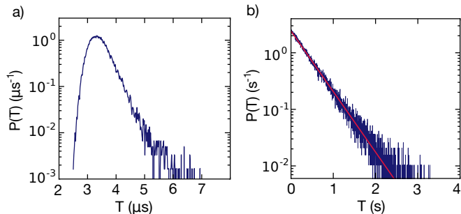
FIG. 4. Probability density function for the transient durations of networks with a) \mathbf{n} = (2, 2, 2) and b) \mathbf{n} = (7, 7, 7) delay elements. Here, a histogram is generated indicating the number of instances that we observe a transient time within T and T + \Delta T , normalized by \Delta T and the total number of observed transient times. It approximates the transient time probability density P(T) , where P(T)\Delta T is the probability of observing a time interval T when \Delta T is small. b) The mean transient duration \langle T \rangle is 0.41 s and the red line shows an exponential fit ( p(T) \propto e^{-\lambda T} ) to the data with exponent \lambda = 2.44 \text{ s}^{-1} .
