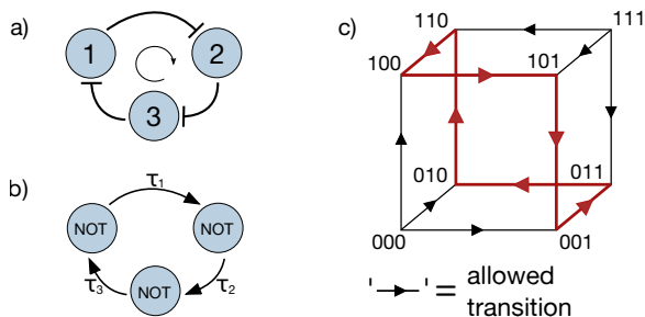
FIG. 1. a) Ring network of N = 3 nodes with inhibitory interactions. b) Description of a) as time-delay autonomous Boolean network. c) State transition diagram of the autonomous Boolean network b) without link delays.
