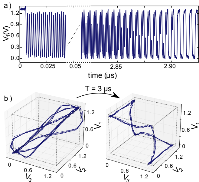
FIG. 2. Temporal evolution of the transient dynamics. a) Waveform of one node in a network with \mathbf{n} = (2, 2, 2) delay elements initialized in the (1, 1, 1) state. The initial nearly-periodic in-phase behavior eventually gives way to out-of-phase oscillations after T \approx 3 \mu\text{s} . b) Corresponding three-dimensional phase portrait of the trajectory, which evolves from in-phase nearly-periodic oscillations (left) to the asymptotic out-of-phase periodic attractor (right).
