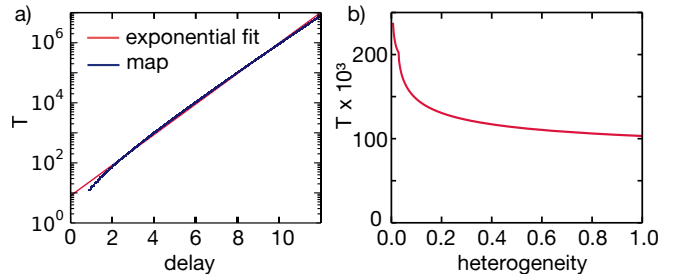
FIG. 7. Transient durations for the map (5) and (6) for N = 3 with no stochastic fluctuations in the time delay ( \xi = 0 ). a) Transient durations as a function of the mean delay \tau for a fixed heterogeneity \Delta = 0.1 , defined by \tau_1 = \tau + \Delta/2 , \tau_2 = \tau and \tau_3 = \tau - \Delta/2 . Differences in initialization timing are not explicitly taken into account, i.e. , \delta_i = 0 . An exponential fit ( T \propto e^{\lambda\tau} ) to the data with exponent \lambda = 1.17 is shown in red. b) Transient durations as a function of delay heterogeneity \Delta for a fixed mean delay \tau = 8 .
