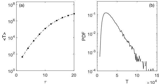
FIG. 8. Transient durations for the map (6) for N = 3 . a) Mean transient duration as a function of the mean delay \tau for \sigma^2 = 10^{-4} . b) Probability density function of the transient duration for \tau = 10 and \sigma^2 = 10^{-4} .
