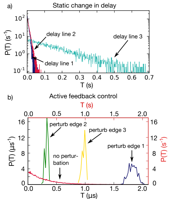
FIG. 6. Transient duration distributions in the presence of heterogeneities and active feedback control. a) Transient duration distributions in a network with \mathbf{n} = (7, 7, 7) delay elements when individually altering the timing of the initial conditions of each node by roughly 100 ps. The mean transient durations when delaying node 1, 2 and 3 are \langle T \rangle = 5.93 ms, \langle T \rangle = 8.05 ms and \langle T \rangle = 151.46 ms, respectively. We collected 30,000 samples for each distribution. b) Transient duration distributions in a network with \mathbf{n} = (6, 6, 6) delay elements, when perturbing the timing of a specific traveling edge. Note, that the time scale for the distribution with no perturbation (red) is seconds.
