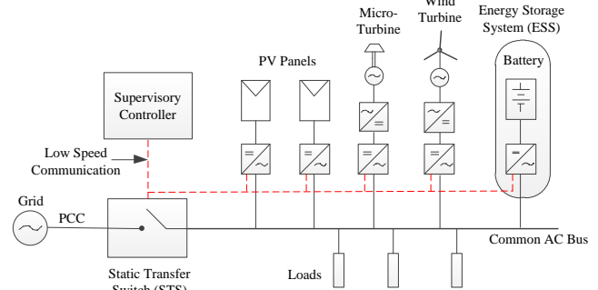
Fig. 1. Microgrid Structure
