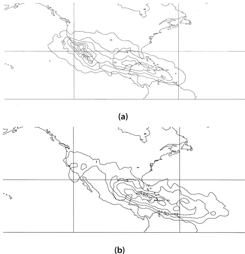
FIG. 4. Origins of the (a) warm and (b) the cold particles. The contour interval is 40 per unit area ( 1^{\circ} \times 1^{\circ} grid box).
