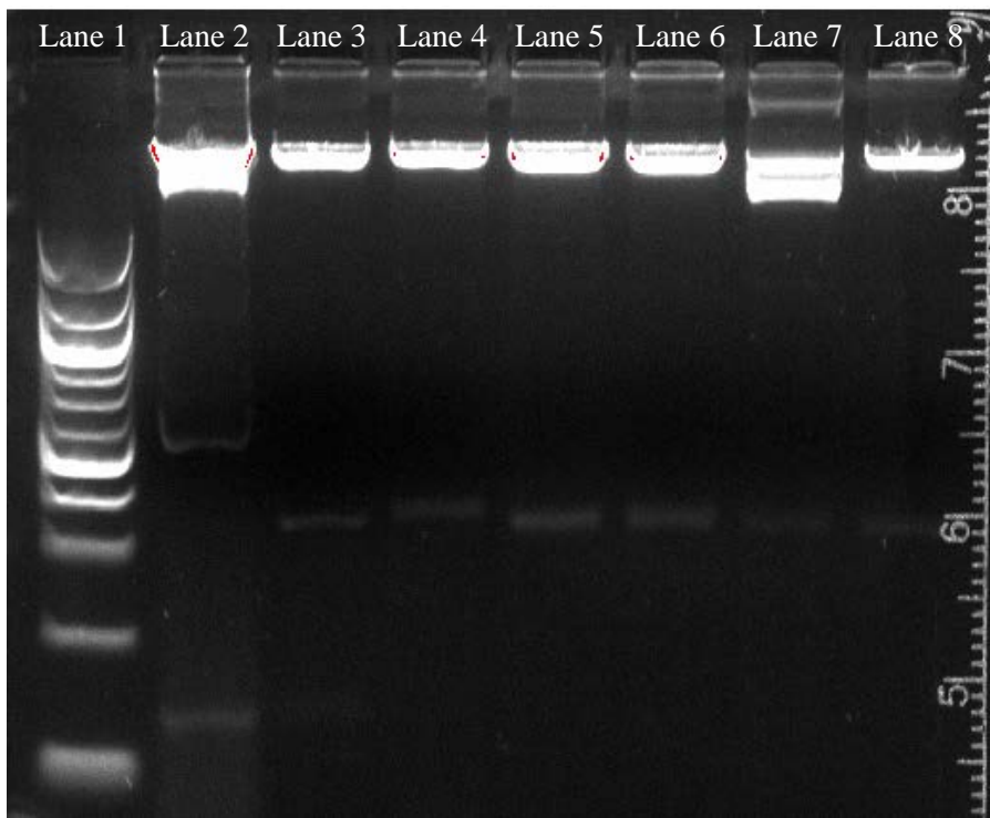
Figure 2. Verification of successful ligation of pJS107 (vector) and nucleotide 532 re-targeting fragment. Lane 1: 100 bp ladder, lane 2: digested pJS107 with Hind III and Bsr GI, and lanes 3-8: potential re-targeted isolates digested with Hind III and Bsr GI.
