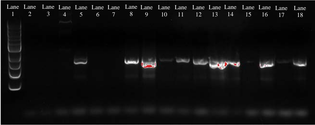
Figure 4. Screening for mutations in CD2311 at nucleotide 532. Lane 1: 1 kb ladder, lane 2: distilled water, lane 3: E. coli DH5 \alpha pNS02, lane 4: E. coli MB3436 pNS02, lane 5: wildtype C. difficile UK1, and lanes 6-18: lincomycin-resistant colonies that were screened for the CD2311 mutant.
