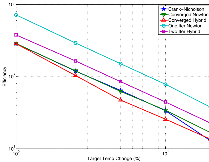
Figure 3.9: Efficiency of the methods for temperature versus number of times steps for the Marshak wave.
