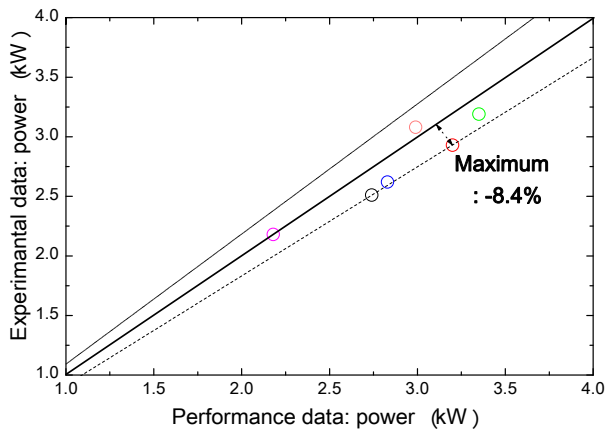
Figure 8. Comparison of power(after refrigerant recharge).
