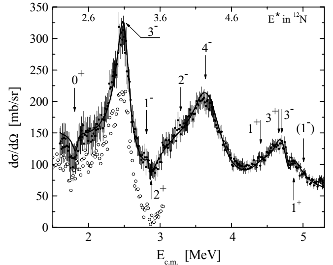
FIG. 3. The zero degree solid target c.m. excitation function and the corresponding R-matrix fit. Zero-degree gas target data (open circles) are also shown. Note that for clarity, the gas target spectrum is shifted down in cross section by a constant amount of 50 mb/sr. Excitation energy E^* is E_{\text{c.m.}} + 0.601 MeV.
