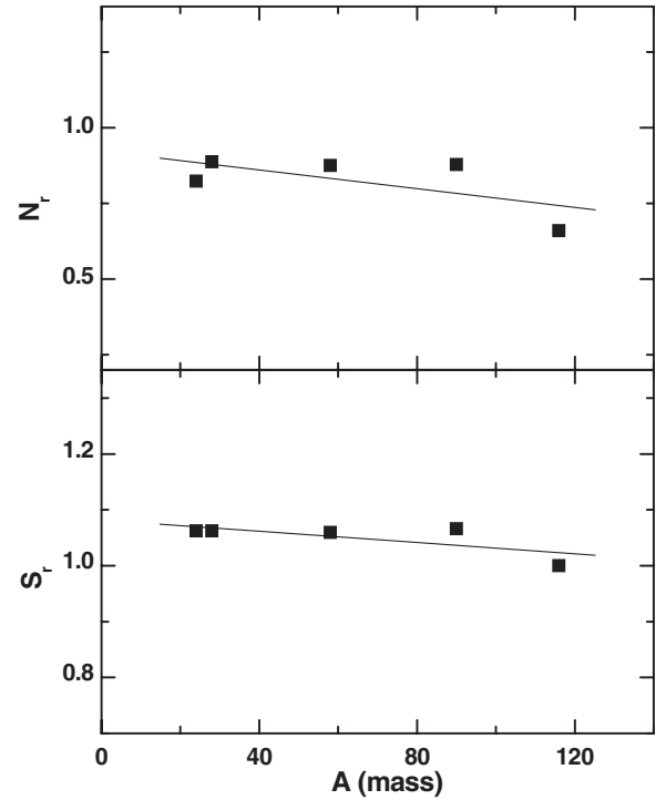
FIG. 4. The target mass number dependence of real normalization ( N_r ) and radius scaling ( S_r ) factors is shown by solid squares. The ^{24}\text{Mg} and ^{28}\text{Si} results are from Ref. [16], and the ^{116}\text{Sn} result is from Ref. [17]. Solid lines are linear fits of the data.
