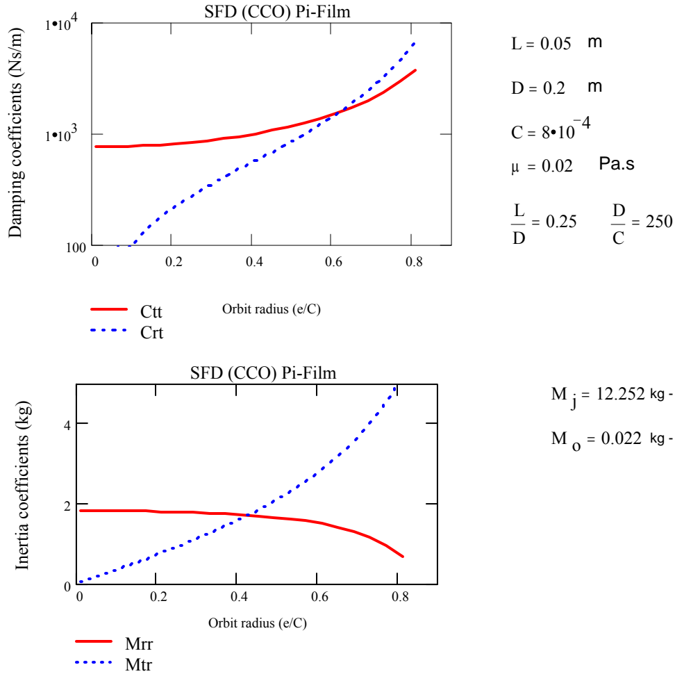
Fig. 6. Open ends SFD force coefficients for circular centered motions. (Short length \pi film model)
