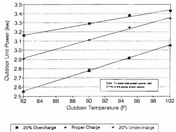
Figure 2. Linear variation of power with respect to temperature for three charging conditions [4].
