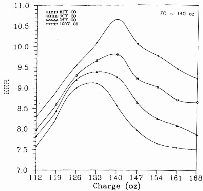
Figure 3. Variation of steady state energy efficiency ratio (EER) with refrigerant charge and temperature.
