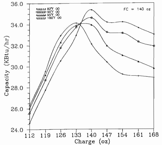
Figure 1. Measured capacity as a function of charge and temperature for a capillary tube expansion air conditioner [4].
