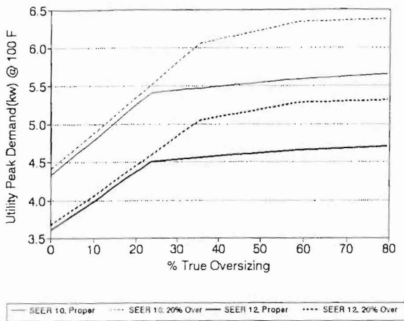
Figure 6. Variation of utility peak demand with oversizing, SEER and refrigerant charge.
