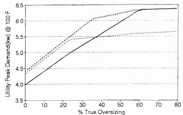
Figure 5. Variation of utility peak demand at 100 F outdoor temperature with percent oversizing and refrigerant charging.
