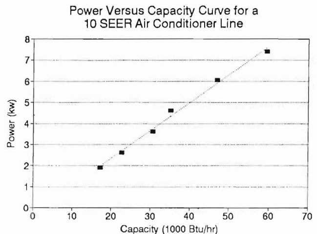
Figure 4. Power demand as a function of capacity for a line of SEER 10 air conditioners.
