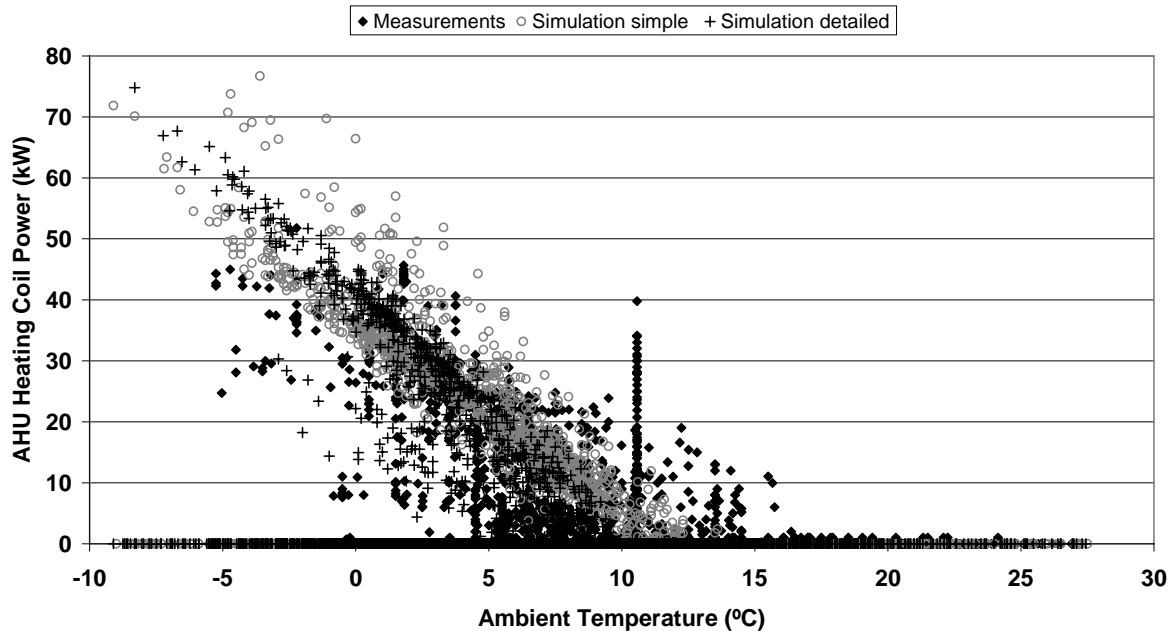
Figure 4: Energy signature graph of AHU heating coil power for 1 st January – 25 th May
