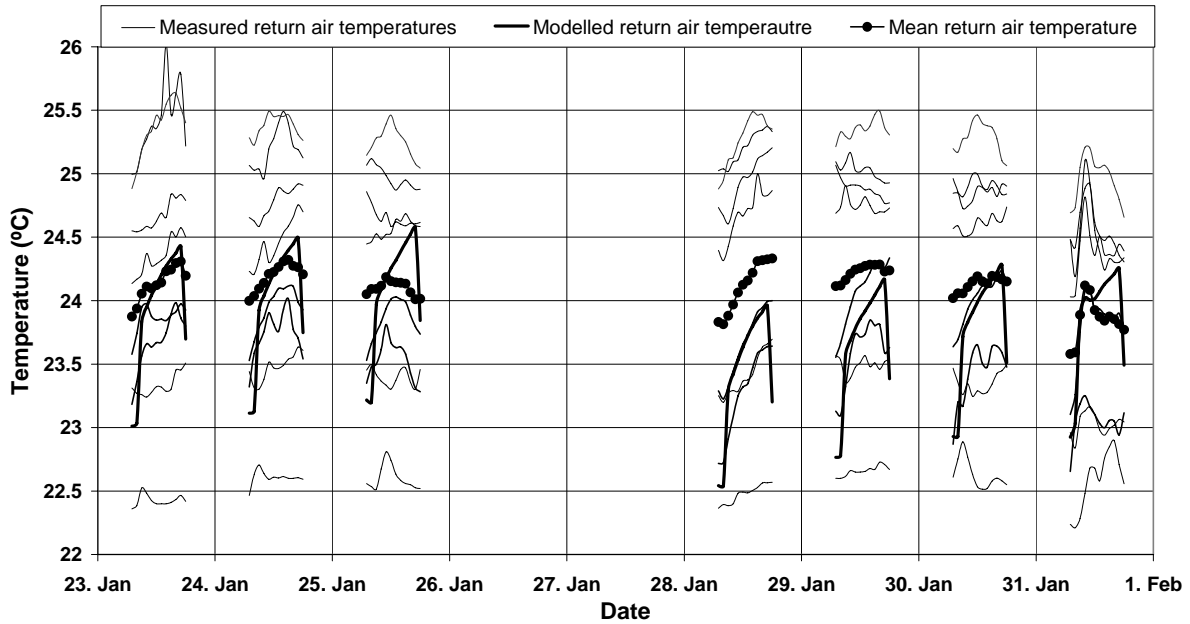
Figure 3: Comparison between measured and simulated return air temperatures for 23 rd January– 1 st February 2008 only recorded when fans are operating
