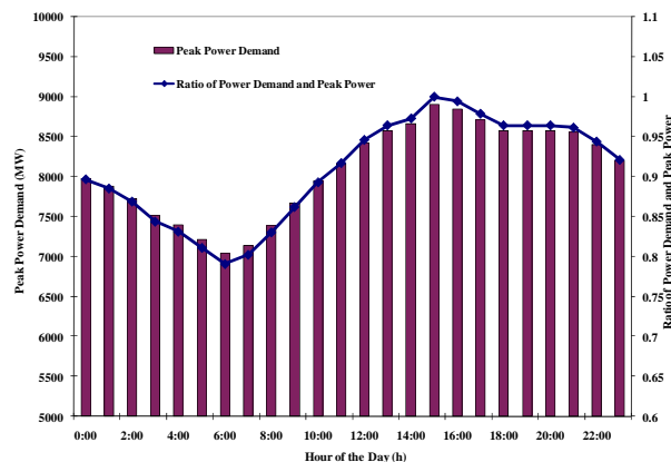
Figure 1. Peak power demand profile for a typical summer day in Kuwait
