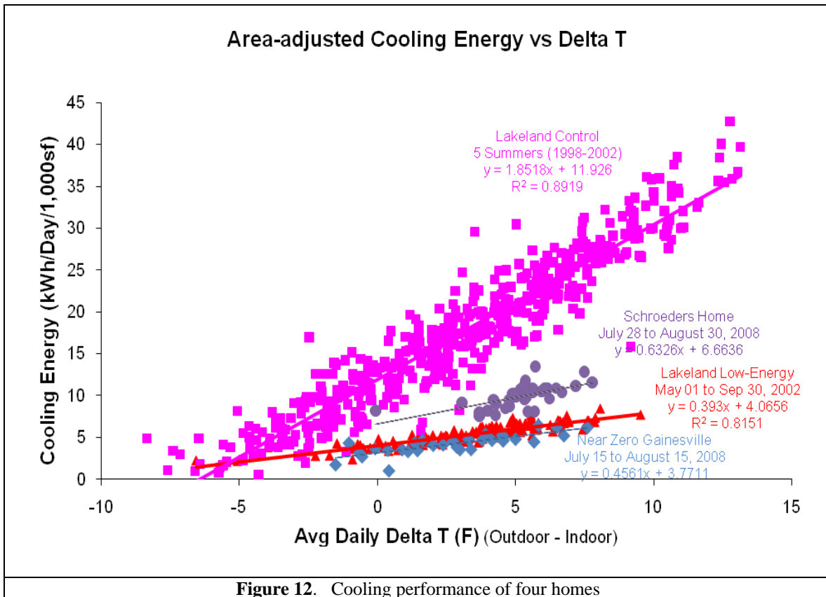
Figure 12. Cooling performance of four homes
