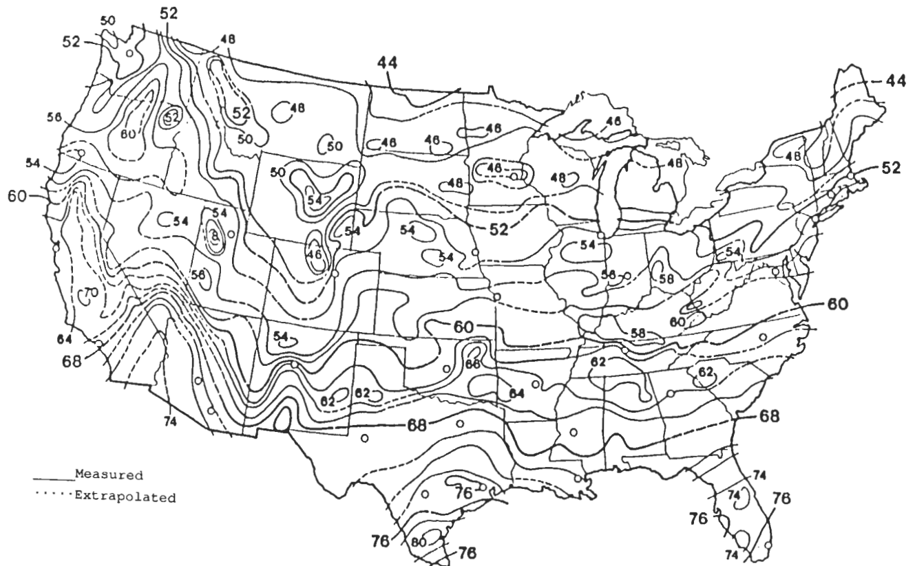
Figure 1. Distribution of Groundwater Temperatures Measured in Nonthermal Wells Ranging in Depth from 50 to 150 ft ( ^\circ\text{F} ) Source: National Water Well Association.
