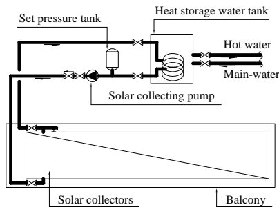
Fig. 24 Flow diagram of individual hot water supply system
