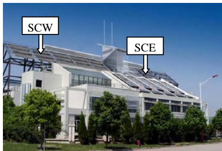
Fig. 17 The external appearance of the green building integrated with solar collectors
