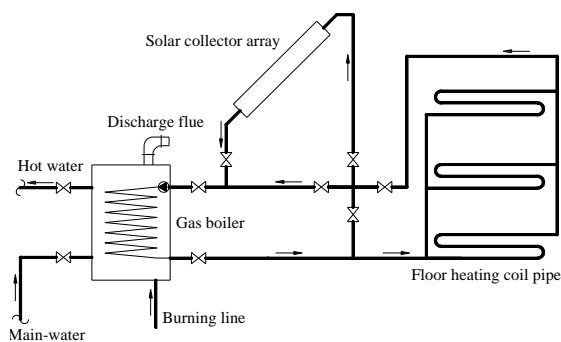
Fig. 15 Schematic drawing of the energy system
