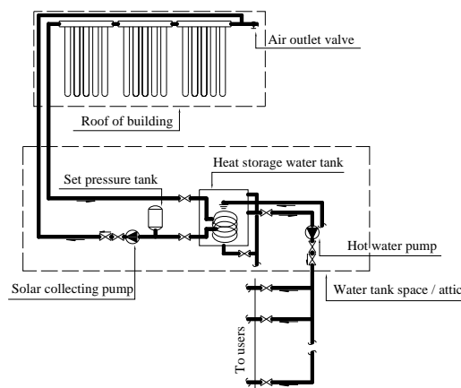
Fig. 22 Flow diagram of central hot water supply system
