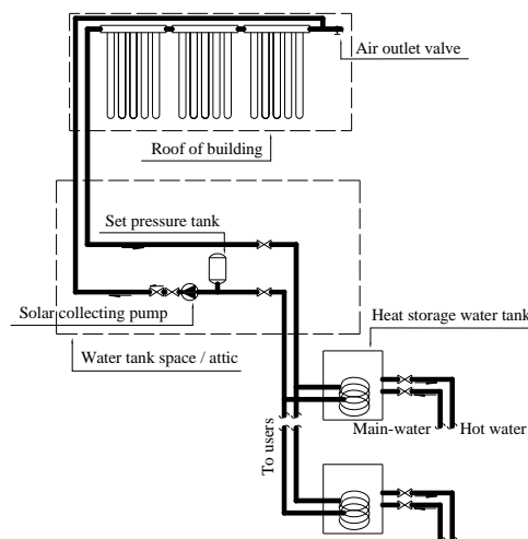
Fig. 23 Flow diagram of central-individual hot water supply system
