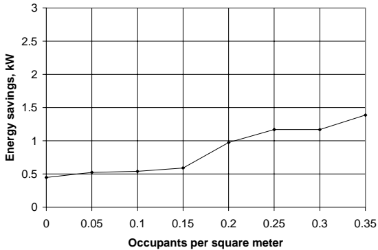
Figure 6: Cooling energy savings for energy-optimal strategy.
