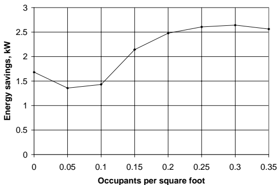
Figure 7: Heating energy savings for energy-optimal strategy.
