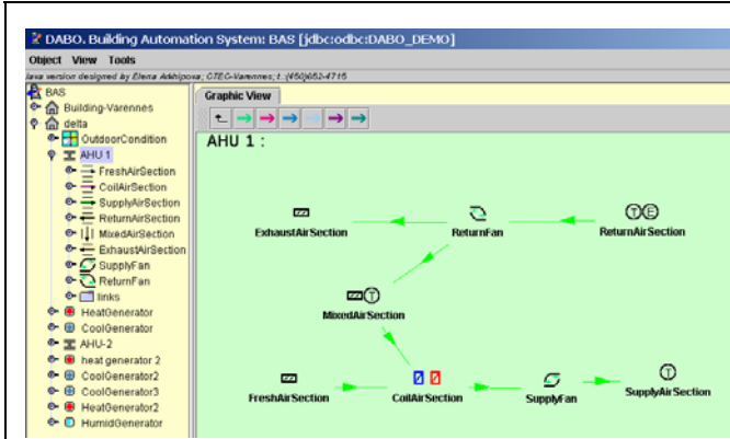
Figure 5: DABO-AHU configuration
