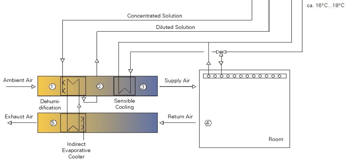
Figure 2: Solar Liquid Desiccant Cooling System LDCS
