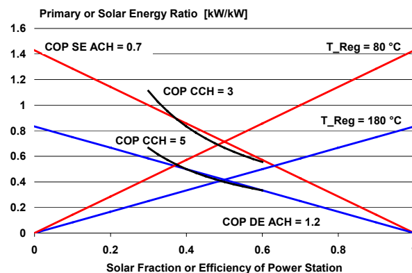
Figure 1: Comparison of primary energy ratio for different solar and conventional cooling technologies.
