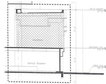
Figure 5. Holdroom section
