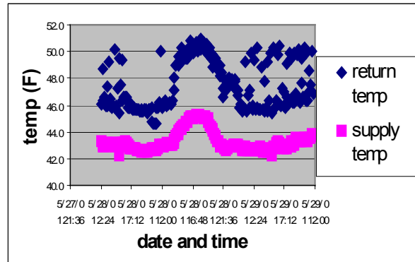
Figure 9: Building chilled water supply and return temperatures
