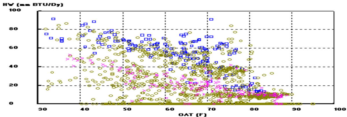
Figure 11: Hot water consumption (□--before CC, o--between CC implementation and follow-up, x--after CC follow-up)
