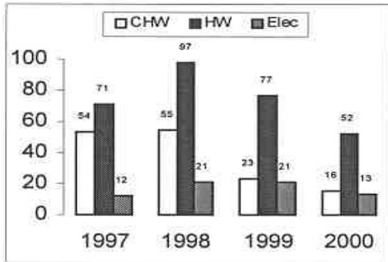
Figure 5: Energy savings after CC implementation
