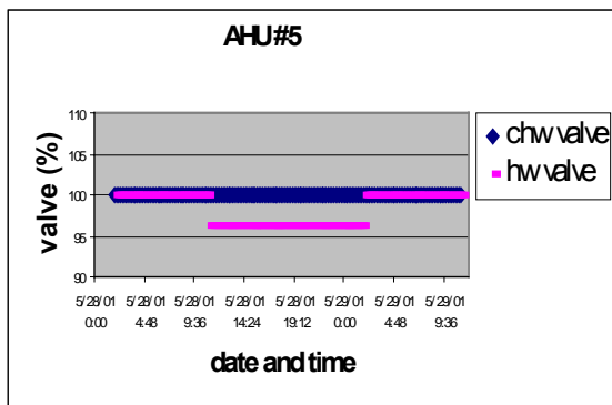
Figure 7: Simultaneous cooling and heating on AHU#5
