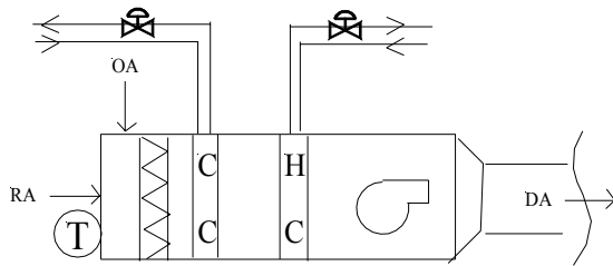
Figure 2: System diagram typical of the 13 large AHUs
