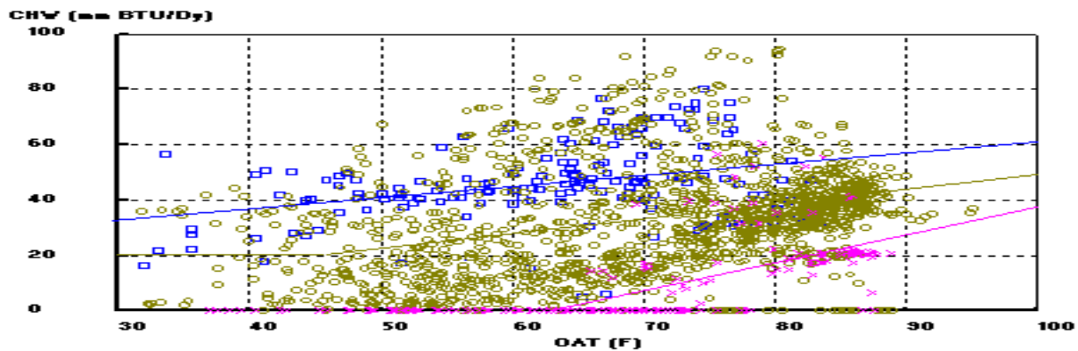
Figure 10: Chilled water consumption (□--before CC, o--between CC implementation and follow-up, x--after CC follow-up)
