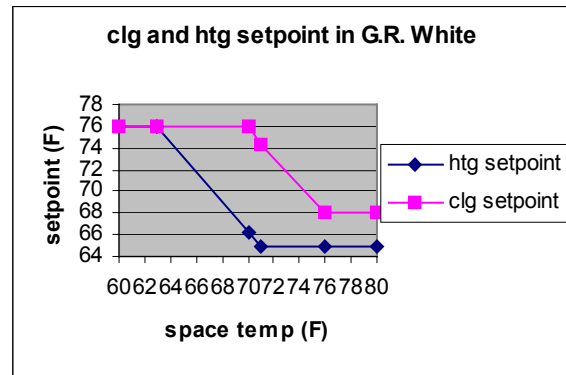
Figure 6: cooling and heating setpoints when there was no event
