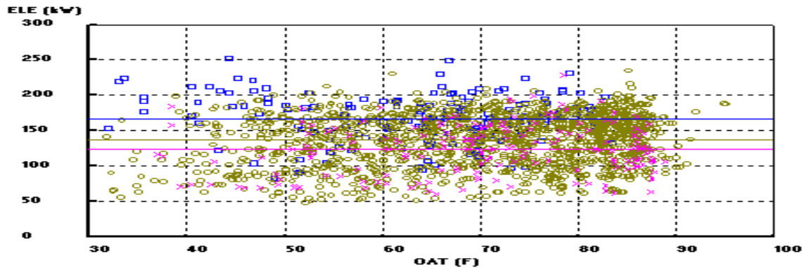
Figure 12: Electricity consumption □--before CC, o--between CC implementation and follow-up, x--after CC follow-up)
