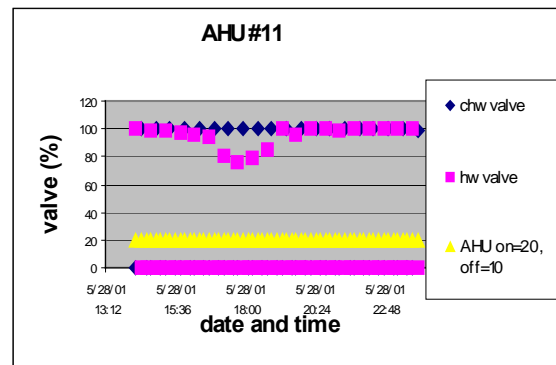
Figure 8: Simultaneous cooling and heating on AHU#11
